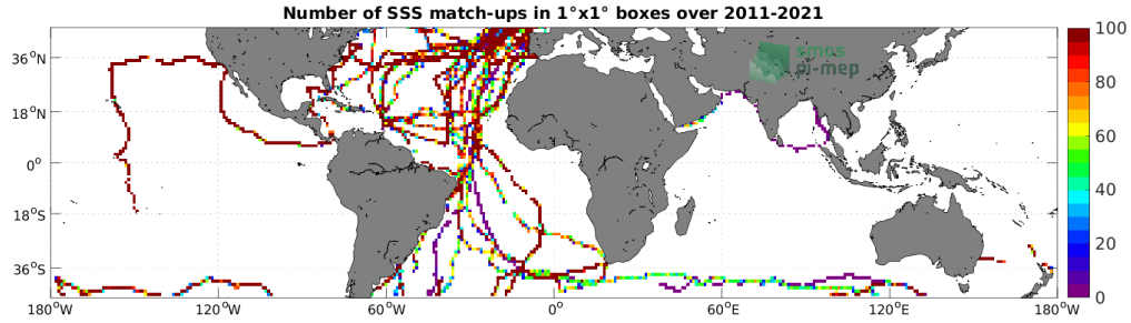
Figure 4: Number of SSS match-ups between TSG (GOSUD-Sailing-ship) SSS and the SMAP SSS L4 OI v1 - 7 Days (IPRC) SSS product for the Mid-Low Latitudes 45N-45S Pi-MEP region over 1^\circ \times 1^\circ boxes and for the full satellite product period.
