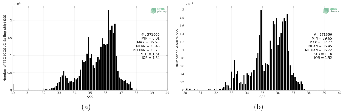
Figure 2: Histograms of SSS from TSG (GOSUD-Sailing-ship) (a) and SMAP SSS L4 OI v1 - 7 Days (IPRC) (b) considering all match-up pairs per bins of 0.1 over the Mid-Low Latitudes 45N-45S Pi-MEP region and for the full satellite product period.
