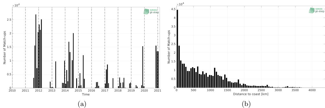
Figure 1: Number of match-ups between TSG (GOSUD-Sailing-ship) and SMAP SSS L4 OI v1 - 7 Days (IPRC) SSS as a function of time (a) and as function of the distance to coast (b) over the Mid-Low Latitudes 45N-45S Pi-MEP region and for the full satellite product period.
