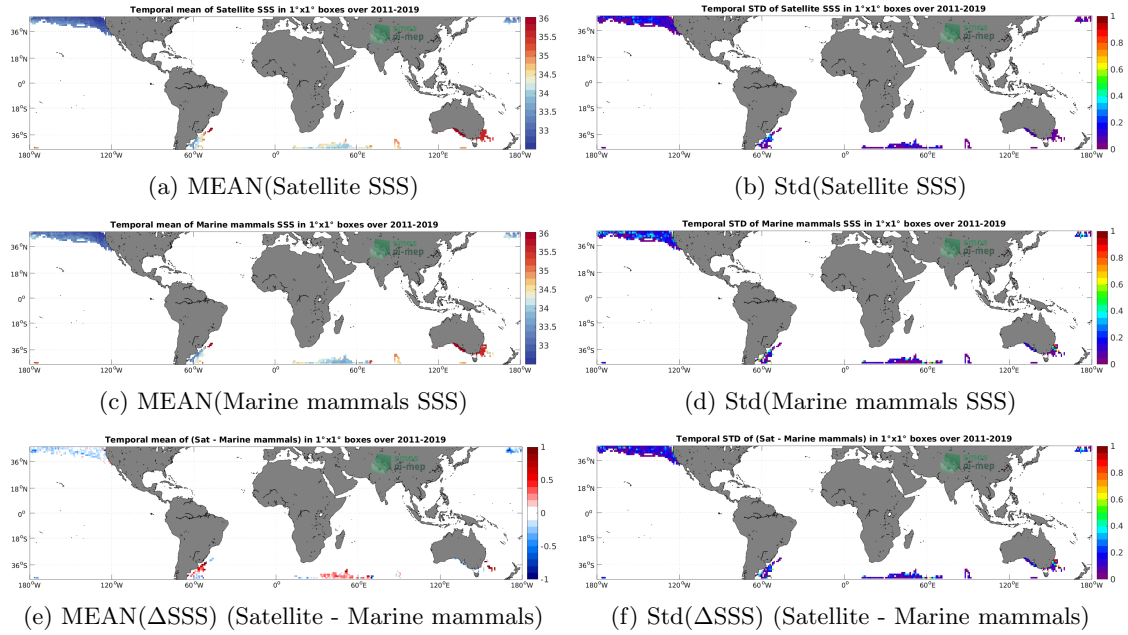
Figure 6: Temporal mean (left) and Std (right) of SSS from SMAP SSS L4 OI v1 - 7 Days (IPRC) (top), Marine mammals (middle), and of \Delta SSS (Satellite - Marine mammals). Only match-up pairs are used to generate these maps.
