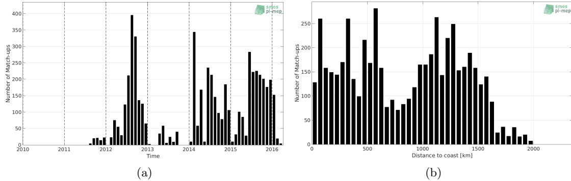
Figure 1: Number of match-ups between Marine mammals and SMAP SSS L4 OI v1 - 7 Days (IPRC) SSS as a function of time (a) and as function of the distance to coast (b) over the Mid-Low Latitudes 45N-45S Pi-MEP region and for the full satellite product period.
