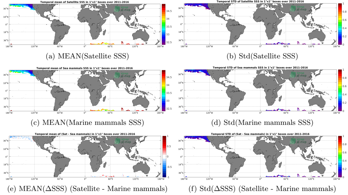
Figure 6: Temporal mean (left) and Std (right) of SSS from SMAP SSS L4 OI v1 - 7 Days (IPRC) (top), Marine mammals (middle), and of \Delta SSS (Satellite - Marine mammals). Only match-up pairs are used to generate these maps.
