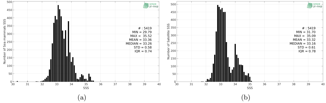
Figure 2: Histograms of SSS from Marine mammals (a) and SMAP SSS L4 OI v1 - 7 Days (IPRC) (b) considering all match-up pairs per bins of 0.1 over the Mid-Low Latitudes 45N-45S Pi-MEP region and for the full satellite product period.
