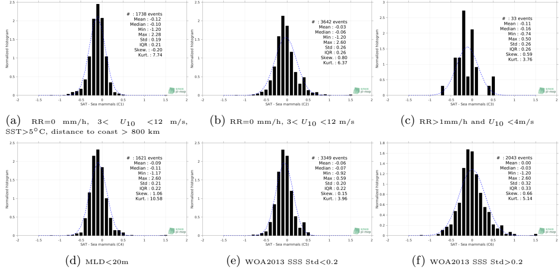
Figure 13: Normalized histogram of \Delta SSS (SMAP SSS L4 OI v1 - 7 Days (IPRC) - Marine mammals) for 6 different subdatasets corresponding to: RR=0 mm/h, 3 < U_{10} < 12 m/s, SST>5°C, distance to coast > 800 km (a), RR=0 mm/h, 3 < U_{10} < 12 m/s (b), RR>1mm/h and U_{10} < 4 m/s (c), MLD<20m (d), WOA2013 SSS Std<0.2 (e), WOA2013 SSS Std>0.2 (f).
