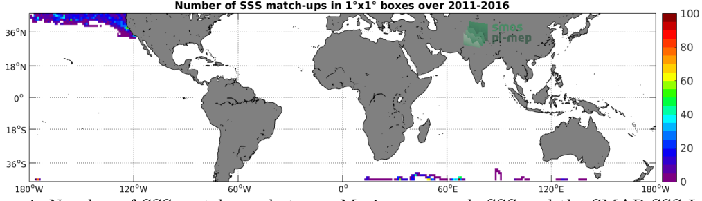
Figure 4: Number of SSS match-ups between Marine mammals SSS and the SMAP SSS L4 OI v1 - 7 Days (IPRC) SSS product for the Mid-Low Latitudes 45N-45S Pi-MEP region over 1^\circ \times 1^\circ boxes and for the full satellite product period.
