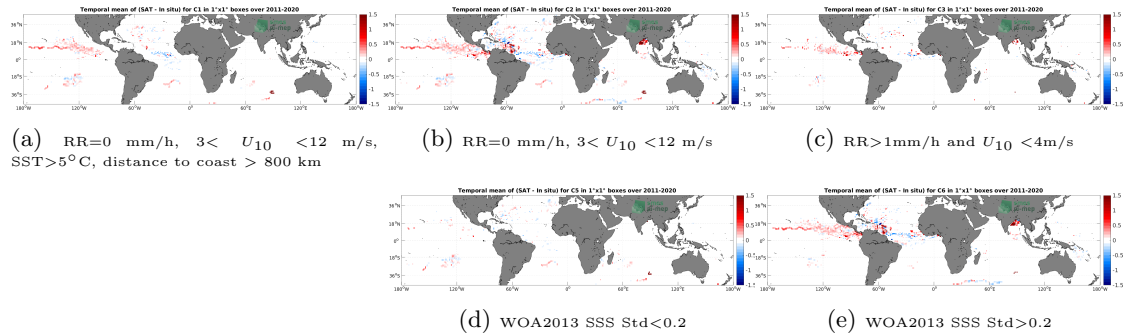
Figure 11: Temporal mean gridded over spatial boxes of size 1^\circ \times 1^\circ of \Delta SSS (SMAP SSS L4 OI v1 - 7 Days (IPRC) - Surface drifters) for 5 different subdatasets corresponding to:RR=0 mm/h, 3 < U_{10} < 12 m/s, SST>5°C, distance to coast > 800 km (a), RR=0 mm/h, 3 < U_{10} < 12 m/s (b), RR>1mm/h and U_{10} < 4 m/s (c), WOA2013 SSS Std<0.2 (d), WOA2013 SSS Std>0.2 (e).
