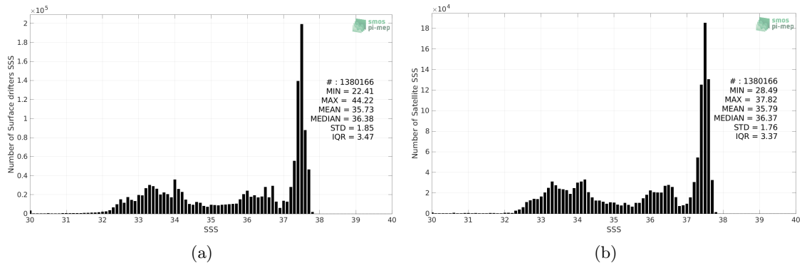
Figure 2: Histograms of SSS from Surface drifters (a) and SMAP SSS L4 OI v1 - 7 Days (IPRC) (b) considering all match-up pairs per bins of 0.1 over the Mid-Low Latitudes 45N-45S Pi-MEP region and for the full satellite product period.
