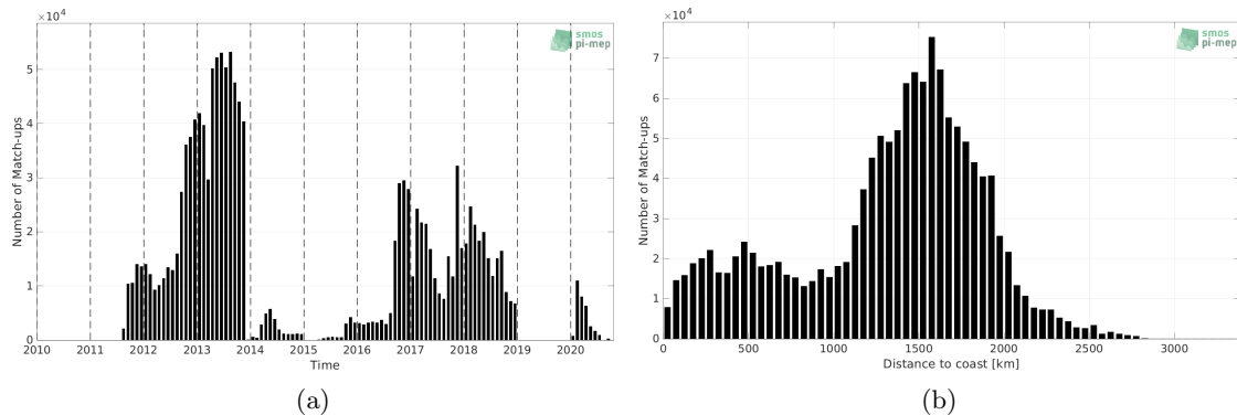
Figure 1: Number of match-ups between Surface drifters and SMAP SSS L4 OI v1 - 7 Days (IPRC) SSS as a function of time (a) and as function of the distance to coast (b) over the Mid-Low Latitudes 45N-45S Pi-MEP region and for the full satellite product period.
