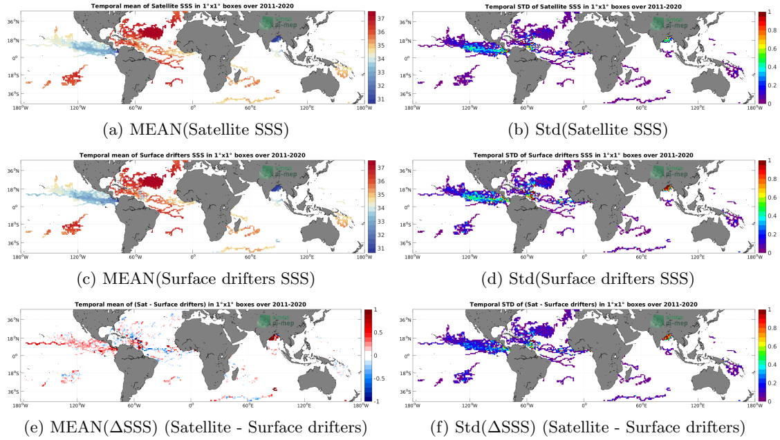
Figure 5: Temporal mean (left) and Std (right) of SSS from SMAP SSS L4 OI v1 - 7 Days (IPRC) (top), Surface drifters (middle), and of \Delta SSS (Satellite - Surface drifters). Only match-up pairs are used to generate these maps.
