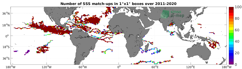
Figure 3: Number of SSS match-ups between Surface drifters SSS and the SMAP SSS L4 OI v1 - 7 Days (IPRC) SSS product for the Mid-Low Latitudes 45N-45S Pi-MEP region over 1^\circ \times 1^\circ boxes and for the full satellite product period.
