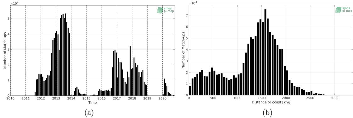
Figure 1: Number of match-ups between Surface drifters and SMAP SSS L4 OI v1 - 7day (IPRC) SSS as a function of time (a) and as function of the distance to coast (b) over the Mid-Low Latitudes 45N-45S Pi-MEP region and for the full satellite product period.
