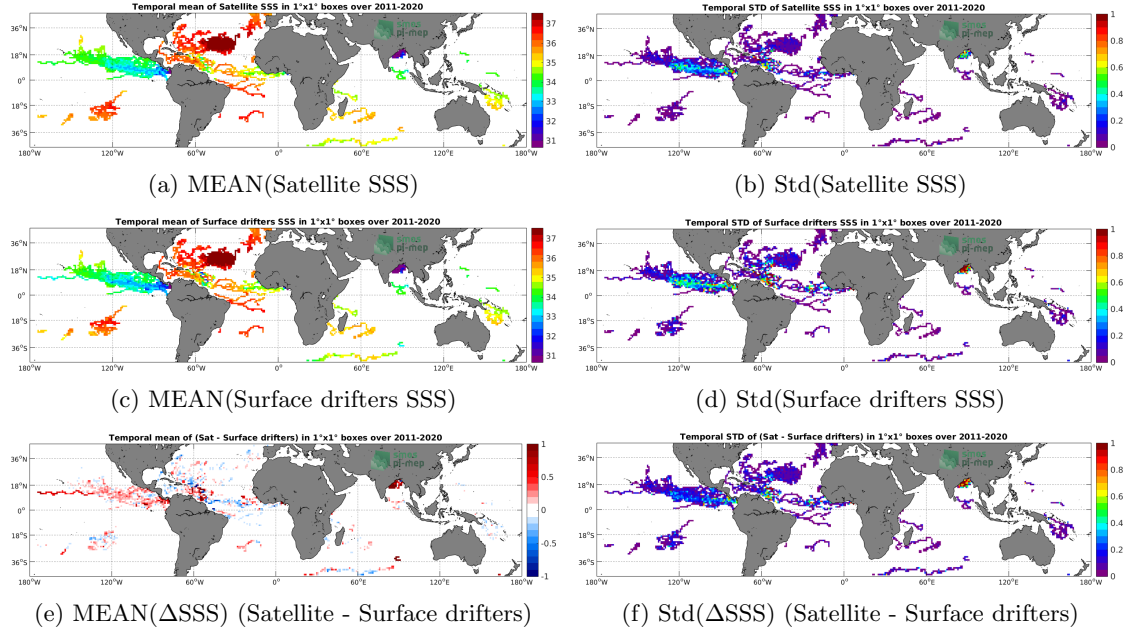
Figure 5: Temporal mean (left) and Std (right) of SSS from SMAP SSS L4 OI v1 - 7day (IPRC) (top), Surface drifters (middle), and of \Delta SSS (Satellite - Surface drifters). Only match-up pairs are used to generate these maps.
