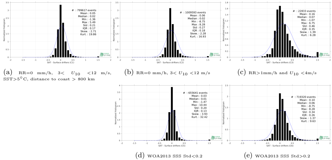
Figure 12: Normalized histogram of \Delta SSS (SMAP SSS L4 OI v1 - 7day (IPRC) - Surface drifters) for 5 different subdatasets corresponding to: RR=0 mm/h, 3 < U_{10} < 12 m/s, SST > 5^\circ C , distance to coast > 800 km (a), RR=0 mm/h, 3 < U_{10} < 12 m/s (b), RR > 1 mm/h and U_{10} < 4 m/s (c), WOA2013 SSS Std < 0.2 (d), WOA2013 SSS Std > 0.2 (e).
