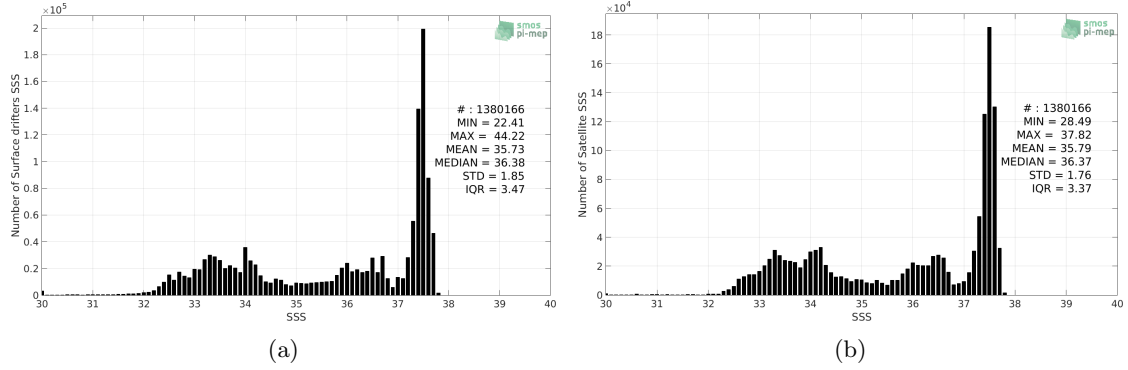
Figure 2: Histograms of SSS from Surface drifters (a) and SMAP SSS L4 OI v1 - 7day (IPRC) (b) considering all match-up pairs per bins of 0.1 over the Mid-Low Latitudes 45N-45S Pi-MEP region and for the full satellite product period.
