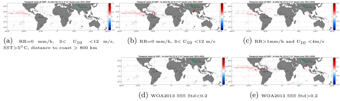
Figure 11: Temporal mean gridded over spatial boxes of size 1^\circ \times 1^\circ of \Delta SSS (SMAP SSS L4 OI v1 - 7day (IPRC) - Surface drifters) for 5 different subdatasets corresponding to: RR=0 mm/h, 3 < U_{10} < 12 m/s, SST > 5^\circ C , distance to coast > 800 km (a), RR=0 mm/h, 3 < U_{10} < 12 m/s (b), RR > 1 mm/h and U_{10} < 4 m/s (c), WOA2013 SSS Std < 0.2 (d), WOA2013 SSS Std > 0.2 (e).
