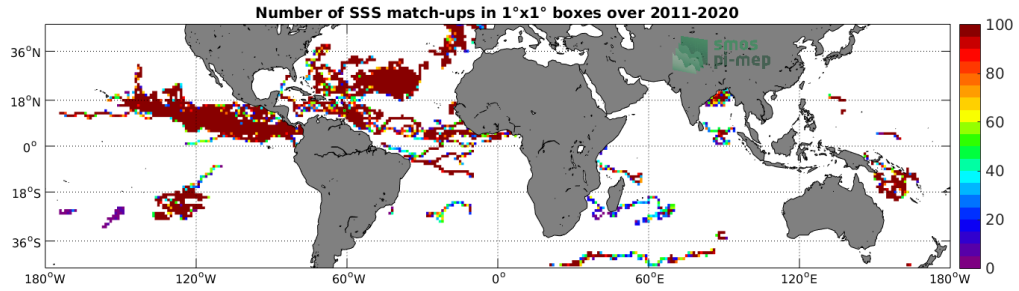
Figure 3: Number of SSS match-ups between Surface drifters SSS and the SMAP SSS L4 OI v1 - 7day (IPRC) SSS product for the Mid-Low Latitudes 45N-45S Pi-MEP region over 1^\circ \times 1^\circ boxes and for the full satellite product period.
