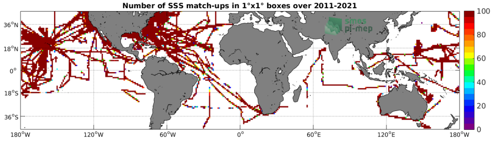
Figure 4: Number of SSS match-ups between TSG (SAMOS) SSS and the SMAP SSS L4 OI v1 - Monthly (IPRC) SSS product for the Mid-Low Latitudes 45N-45S Pi-MEP region over 1^\circ \times 1^\circ boxes and for the full satellite product period.
