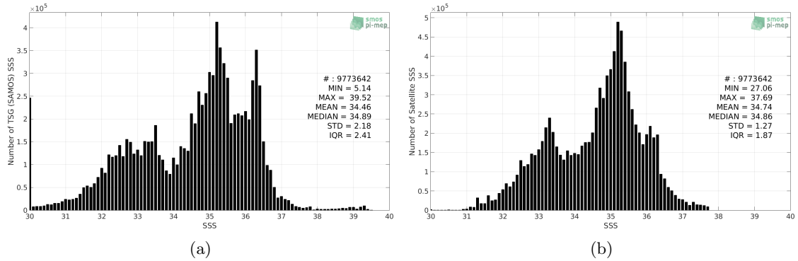
Figure 2: Histograms of SSS from TSG (SAMOS) (a) and SMAP SSS L4 OI v1 - Monthly (IPRC) (b) considering all match-up pairs per bins of 0.1 over the Mid-Low Latitudes 45N-45S Pi-MEP region and for the full satellite product period.
