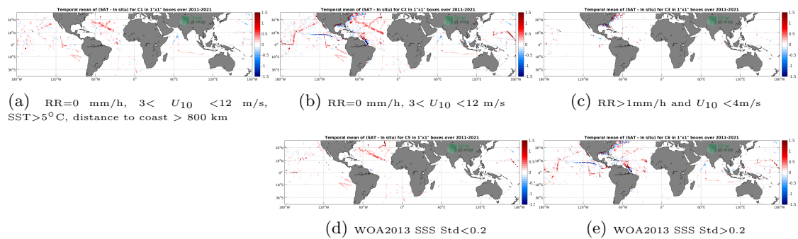
Figure 12: Temporal mean gridded over spatial boxes of size 1^\circ \times 1^\circ of \Delta SSS (SMAP SSS L4 OI v1 - Monthly (IPRC) - TSG (SAMOS)) for 5 different subdatasets corresponding to: RR=0 mm/h, 3 < U_{10} < 12 m/s, SST > 5°C, distance to coast > 800 km (a), RR=0 mm/h, 3 < U_{10} < 12 m/s (b), RR > 1mm/h and U_{10} < 4 m/s (c), WOA2013 SSS Std < 0.2 (d), WOA2013 SSS Std > 0.2 (e).
