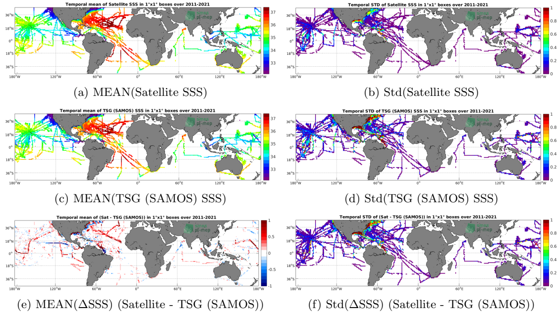
Figure 6: Temporal mean (left) and Std (right) of SSS from SMAP SSS L4 OI v1 - Monthly (IPRC) (top), TSG (SAMOS) (middle), and of \Delta SSS (Satellite - TSG (SAMOS)). Only match-up pairs are used to generate these maps.
