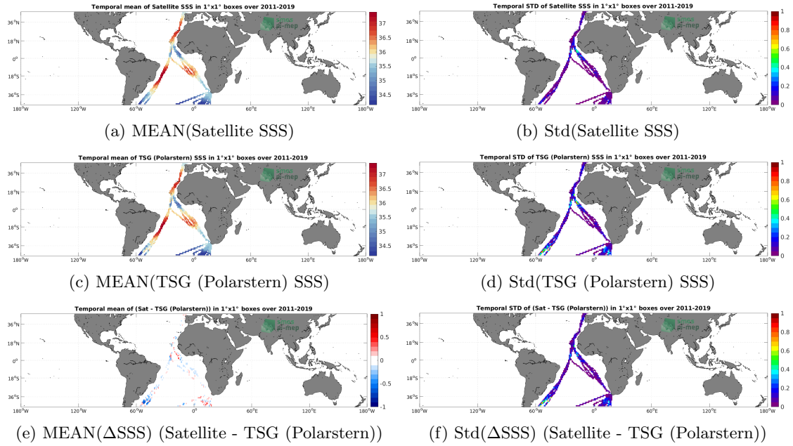
Figure 6: Temporal mean (left) and Std (right) of SSS from SMAP SSS L4 OI v1 - Monthly (IPRC) (top), TSG (Polarstern) (middle), and of \Delta SSS (Satellite - TSG (Polarstern)). Only match-up pairs are used to generate these maps.
