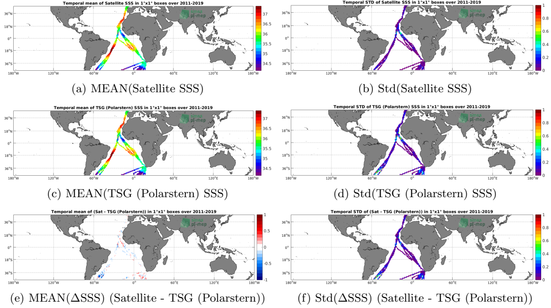
Figure 6: Temporal mean (left) and Std (right) of SSS from SMAP SSS L4 OI v1 - Monthly (IPRC) (top), TSG (Polarstern) (middle), and of \Delta SSS (Satellite - TSG (Polarstern)). Only match-up pairs are used to generate these maps.
