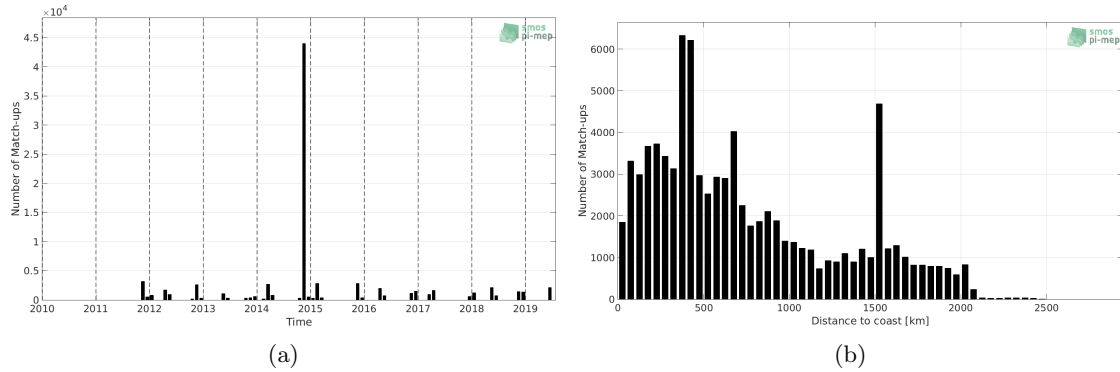
Figure 1: Number of match-ups between TSG (Polarstern) and SMAP SSS L4 OI v1 - Monthly (IPRC) SSS as a function of time (a) and as function of the distance to coast (b) over the Mid-Low Latitudes 45N-45S Pi-MEP region and for the full satellite product period.
