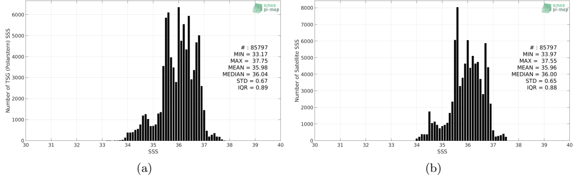
Figure 2: Histograms of SSS from TSG (Polarstern) (a) and SMAP SSS L4 OI v1 - Monthly (IPRC) (b) considering all match-up pairs per bins of 0.1 over the Mid-Low Latitudes 45N-45S Pi-MEP region and for the full satellite product period.
