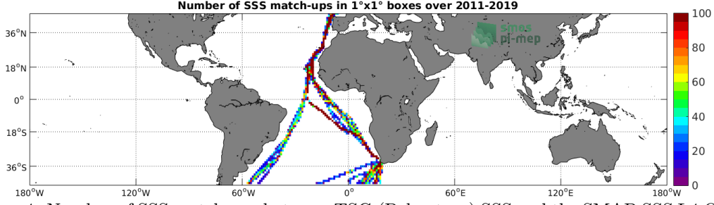
Figure 4: Number of SSS match-ups between TSG (Polarstern) SSS and the SMAP SSS L4 OI v1 - Monthly (IPRC) SSS product for the Mid-Low Latitudes 45N-45S Pi-MEP region over 1^\circ \times 1^\circ boxes and for the full satellite product period.
