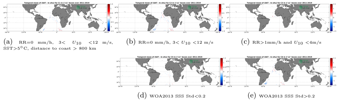
Figure 12: Temporal mean gridded over spatial boxes of size 1^\circ \times 1^\circ of \Delta SSS (SMAP SSS L4 OI v1 - Monthly (IPRC) - TSG (Polarstern)) for 5 different subdatasets corresponding to: RR=0 mm/h, 3 < U_{10} < 12 m/s, SST > 5^\circ C , distance to coast > 800 km (a), RR=0 mm/h, 3 < U_{10} < 12 m/s (b), RR > 1 mm/h and U_{10} < 4 m/s (c), WOA2013 SSS Std < 0.2 (d), WOA2013 SSS Std > 0.2 (e).
