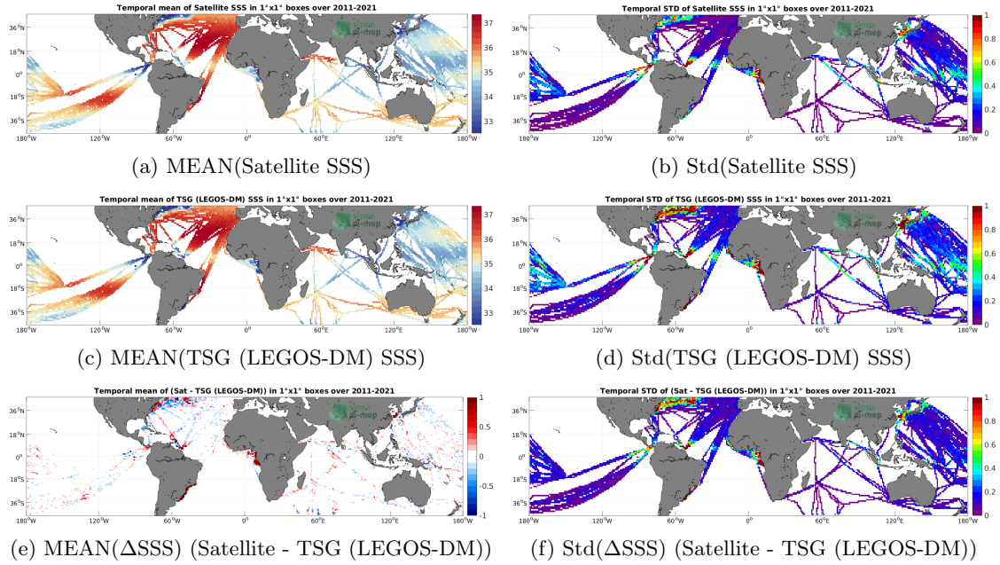
Figure 6: Temporal mean (left) and Std (right) of SSS from SMAP SSS L4 OI v1 - Monthly (IPRC) (top), TSG (LEGOS-DM) (middle), and of \Delta SSS (Satellite - TSG (LEGOS-DM)). Only match-up pairs are used to generate these maps.
