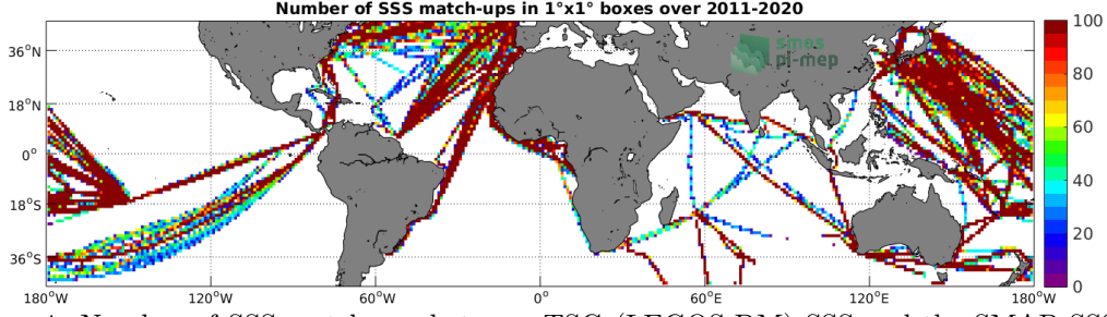
Figure 4: Number of SSS match-ups between TSG (LEGOS-DM) SSS and the SMAP SSS L4 OI v1 - Monthly (IPRC) SSS product for the Mid-Low Latitudes 45N-45S Pi-MEP region over 1^\circ \times 1^\circ boxes and for the full satellite product period.
