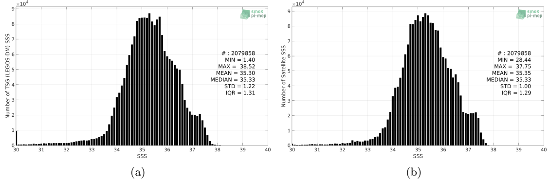
Figure 2: Histograms of SSS from TSG (LEGOS-DM) (a) and SMAP SSS L4 OI v1 - Monthly (IPRC) (b) considering all match-up pairs per bins of 0.1 over the Mid-Low Latitudes 45N-45S Pi-MEP region and for the full satellite product period.
