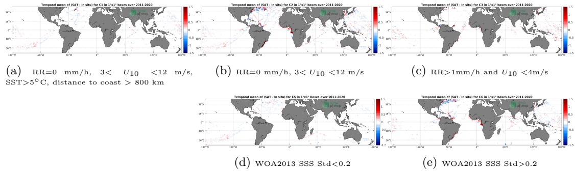
Figure 12: Temporal mean gridded over spatial boxes of size 1^\circ \times 1^\circ of \Delta SSS (SMAP SSS L4 OI v1 - Monthly (IPRC) - TSG (LEGOS-DM)) for 5 different subdatasets corresponding to:RR=0 mm/h, 3 < U_{10} < 12 m/s, SST >5^\circ\text{C} , distance to coast > 800 km (a), RR=0 mm/h, 3 < U_{10} < 12 m/s (b), RR >1 mm/h and U_{10} < 4 m/s (c), WOA2013 SSS Std <0.2 (d), WOA2013 SSS Std >0.2 (e).
