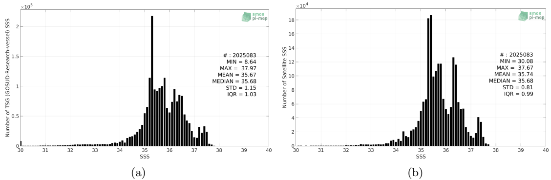
Figure 2: Histograms of SSS from TSG (GOSUD-Research-vessel) (a) and SMAP SSS L4 OI v1 - Monthly (IPRC) (b) considering all match-up pairs per bins of 0.1 over the Mid-Low Latitudes 45N-45S Pi-MEP region and for the full satellite product period.
