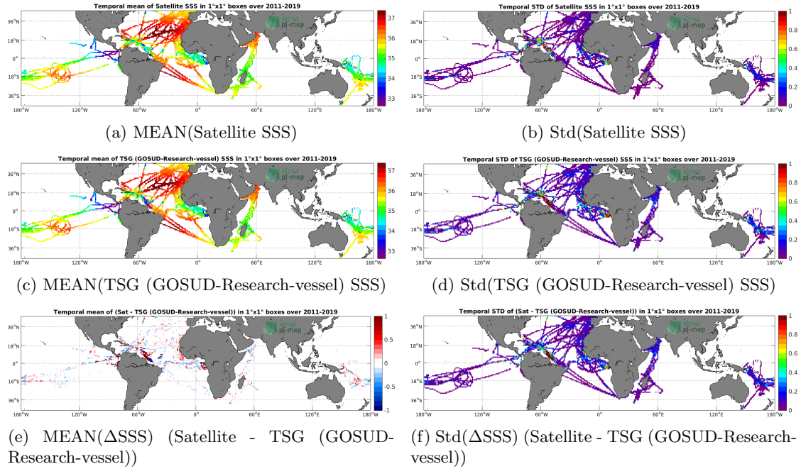
Figure 6: Temporal mean (left) and Std (right) of SSS from SMAP SSS L4 OI v1 - Monthly (IPRC) (top), TSG (GOSUD-Research-vessel) (middle), and of \Delta SSS (Satellite - TSG (GOSUD-Research-vessel)). Only match-up pairs are used to generate these maps.
