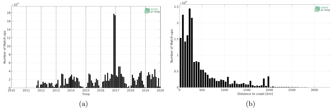
Figure 1: Number of match-ups between TSG (GOSUD-Research-vessel) and SMAP SSS L4 OI v1 - Monthly (IPRC) SSS as a function of time (a) and as function of the distance to coast (b) over the Mid-Low Latitudes 45N-45S Pi-MEP region and for the full satellite product period.
