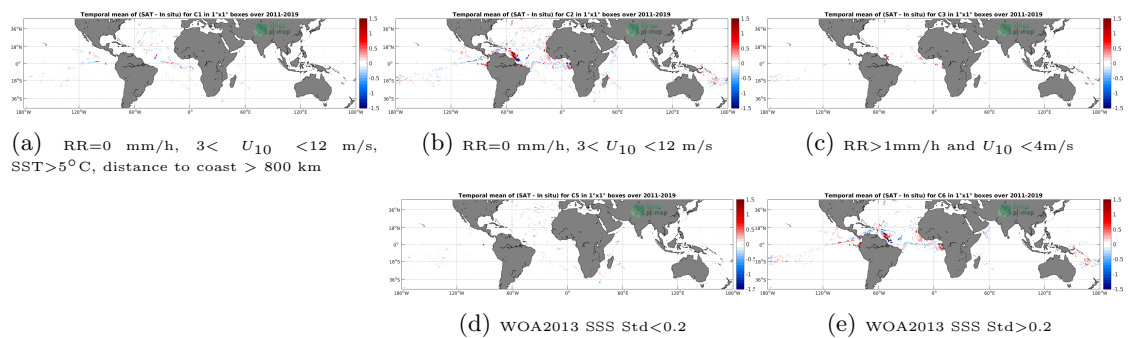
Figure 12: Temporal mean gridded over spatial boxes of size 1^\circ \times 1^\circ of \Delta SSS (SMAP SSS L4 OI v1 - Monthly (IPRC) - TSG (GOSUD-Research-vessel)) for 5 different subdatasets corresponding to: RR=0 mm/h, 3 < U_{10} < 12 m/s, SST > 5°C, distance to coast > 800 km (a), RR=0 mm/h, 3 < U_{10} < 12 m/s (b), RR > 1mm/h and U_{10} < 4 m/s (c), WOA2013 SSS Std < 0.2 (d), WOA2013 SSS Std > 0.2 (e).
