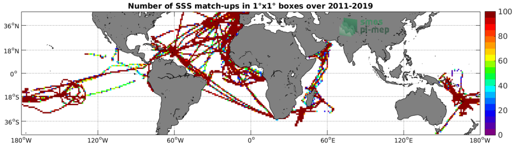
Figure 4: Number of SSS match-ups between TSG (GOSUD-Research-vessel) SSS and the SMAP SSS L4 OI v1 - Monthly (IPRC) SSS product for the Mid-Low Latitudes 45N-45S Pi-MEP region over 1^\circ \times 1^\circ boxes and for the full satellite product period.
