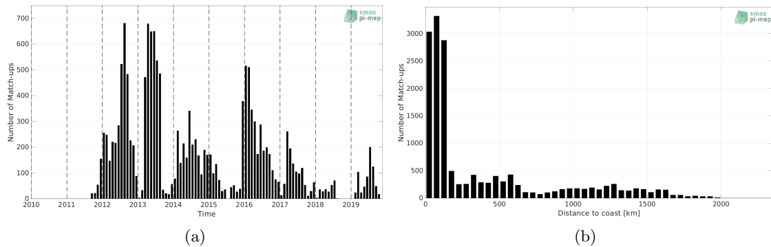
Figure 1: Number of match-ups between Marine mammals and SMAP SSS L4 OI v1 - Monthly (IPRC) SSS as a function of time (a) and as function of the distance to coast (b) over the Mid-Low Latitudes 45N-45S Pi-MEP region and for the full satellite product period.
