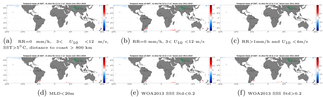
Figure 12: Temporal mean gridded over spatial boxes of size 1^\circ \times 1^\circ of \Delta SSS (SMAP SSS L4 OI v1 - Monthly (IPRC) - Marine mammals) for 6 different subdatasets corresponding to:RR=0 mm/h, 3 < U_{10} < 12 m/s, SST >5^\circ C, distance to coast > 800 km (a), RR=0 mm/h, 3 < U_{10} < 12 m/s (b), RR >1 mm/h and U_{10} < 4 m/s (c),MLD <20 m (d),WOA2013 SSS Std <0.2 (e),WOA2013 SSS Std >0.2 (f).
