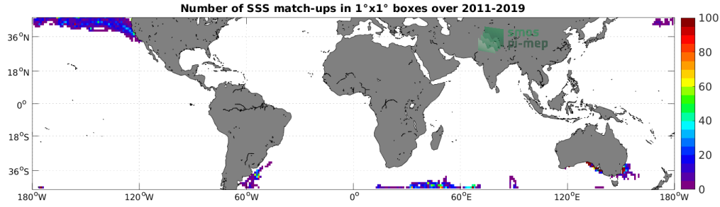
Figure 4: Number of SSS match-ups between Marine mammals SSS and the SMAP SSS L4 OI v1 - Monthly (IPRC) SSS product for the Mid-Low Latitudes 45N-45S Pi-MEP region over 1^\circ \times 1^\circ boxes and for the full satellite product period.
