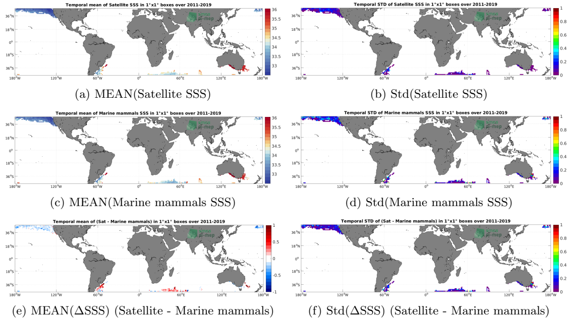
Figure 6: Temporal mean (left) and Std (right) of SSS from SMAP SSS L4 OI v1 - Monthly (IPRC) (top), Marine mammals (middle), and of \Delta SSS (Satellite - Marine mammals). Only match-up pairs are used to generate these maps.
