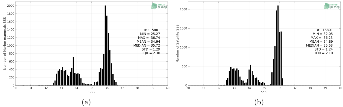
Figure 2: Histograms of SSS from Marine mammals (a) and SMAP SSS L4 OI v1 - Monthly (IPRC) (b) considering all match-up pairs per bins of 0.1 over the Mid-Low Latitudes 45N-45S Pi-MEP region and for the full satellite product period.
