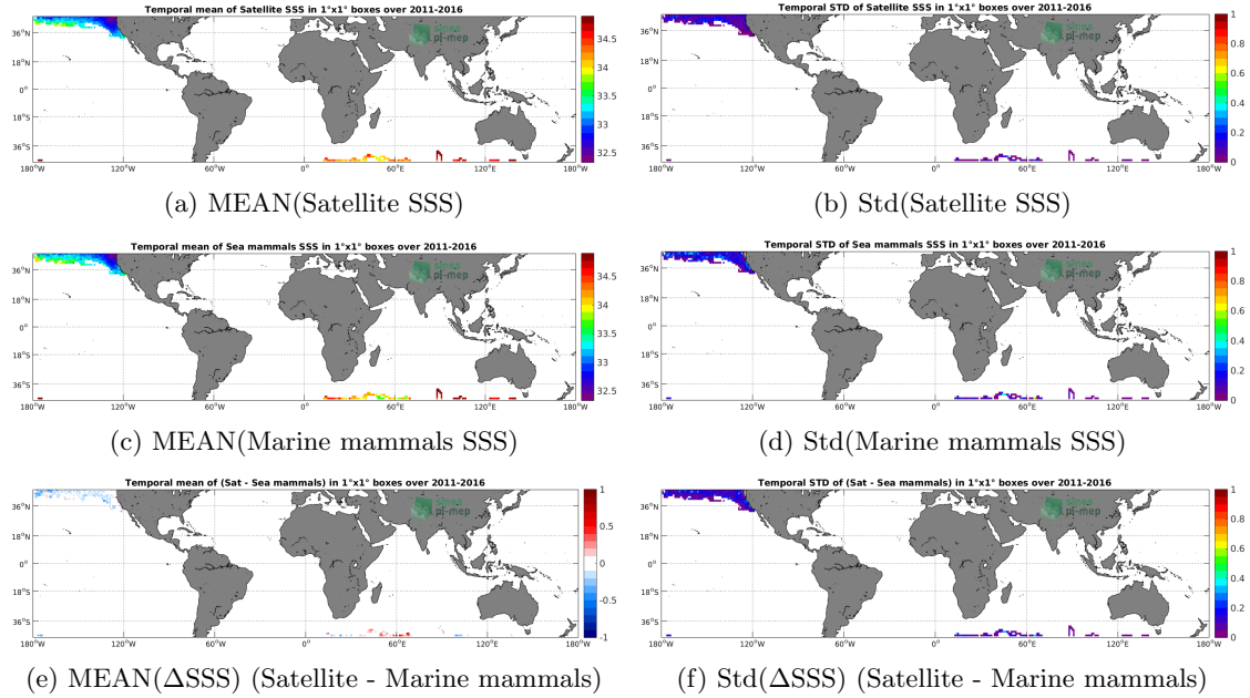
Figure 6: Temporal mean (left) and Std (right) of SSS from SMAP SSS L4 OI v1 - Monthly (IPRC) (top), Marine mammals (middle), and of \Delta SSS (Satellite - Marine mammals). Only match-up pairs are used to generate these maps.
