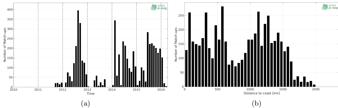
Figure 1: Number of match-ups between Sea mammals and SMAP SSS L4 OI v1 - Monthly (IPRC) SSS as a function of time (a) and as function of the distance to coast (b) over the Mid-Low Latitudes 45N-45S Pi-MEP region and for the full satellite product period.
