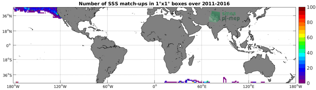
Figure 4: Number of SSS match-ups between Sea mammals SSS and the SMAP SSS L4 OI v1 - Monthly (IPRC) SSS product for the Mid-Low Latitudes 45N-45S Pi-MEP region over 1^\circ \times 1^\circ boxes and for the full satellite product period.
