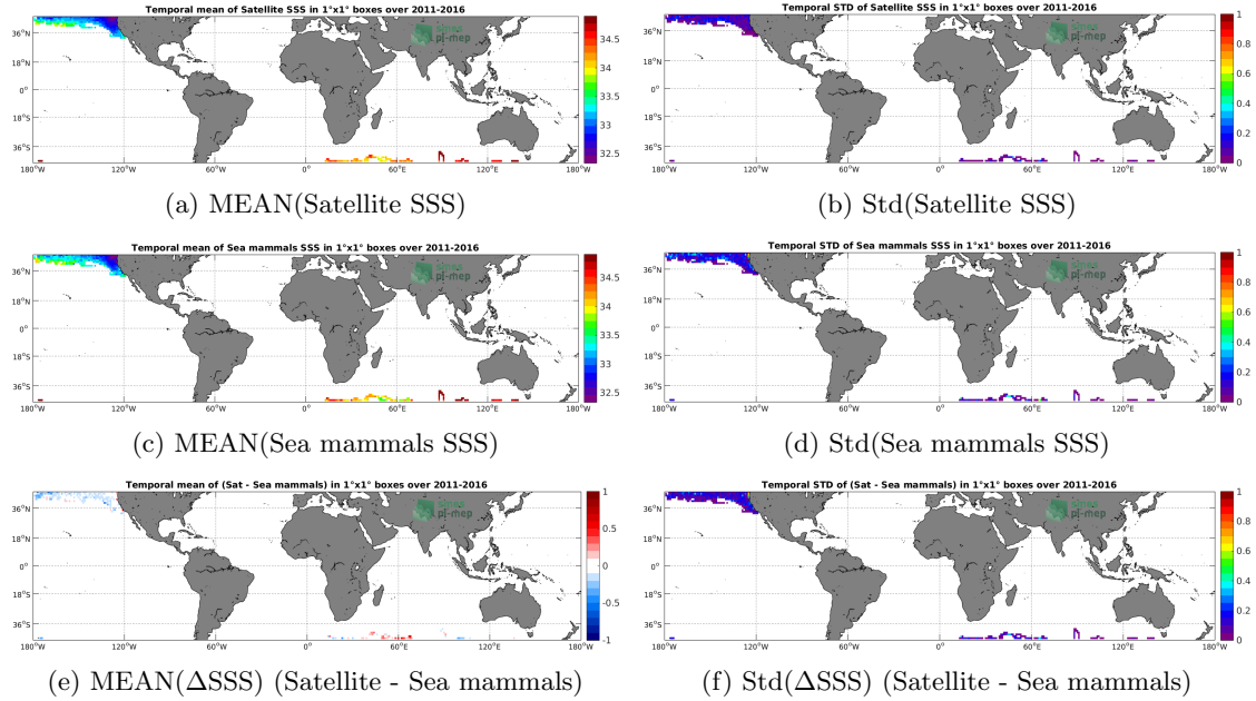
Figure 6: Temporal mean (left) and Std (right) of SSS from SMAP SSS L4 OI v1 - Monthly (IPRC) (top), Sea mammals (middle), and of \Delta SSS (Satellite - Sea mammals). Only match-up pairs are used to generate these maps.
