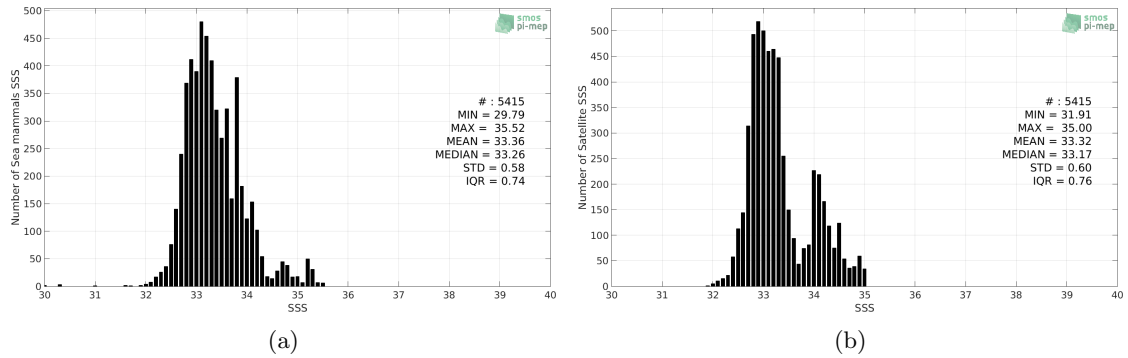
Figure 2: Histograms of SSS from Sea mammals (a) and SMAP SSS L4 OI v1 - Monthly (IPRC) (b) considering all match-up pairs per bins of 0.1 over the Mid-Low Latitudes 45N-45S Pi-MEP region and for the full satellite product period.
