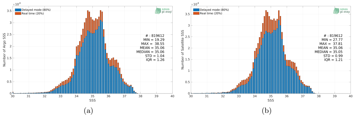
Figure 2: Histograms of SSS from Argo (a) and SMAP SSS L4 OI v1 - Monthly (IPRC) (b) considering all match-up pairs per bins of 0.1 over the Mid-Low Latitudes 45N-45S Pi-MEP region and for the full satellite product period.
