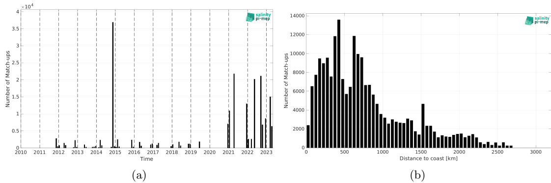
Figure 2: Number of match-ups between TSG (Polarstern) and SMAP SSS L4 OI v3 - Monthly (ESR) SSS as a function of time (a) and as function of the distance to coast (b) over the Mid-Low Latitudes 45N-45S Pi-MEP region and for the full satellite product period.
