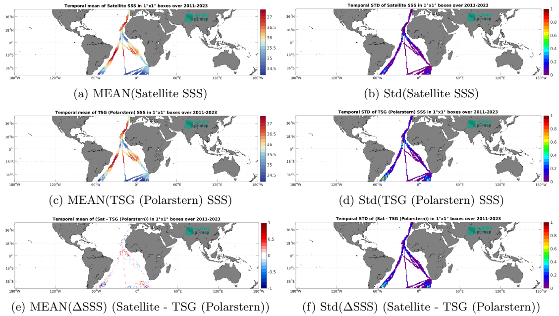
Figure 7: Temporal mean (left) and Std (right) of SSS from SMAP SSS L4 OI v3 - Monthly (ESR) (top), TSG (Polarstern) (middle), and of \Delta SSS (Satellite - TSG (Polarstern)). Only match-up pairs are used to generate these maps.
