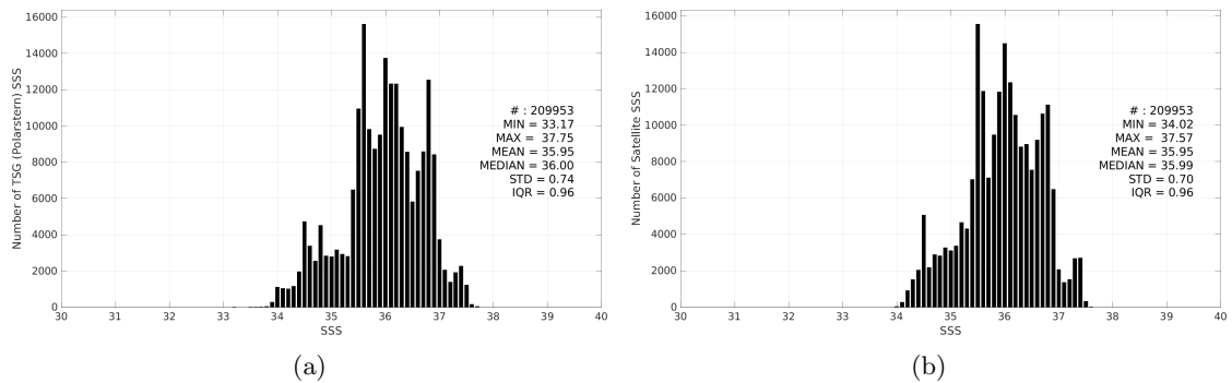
Figure 3: Histograms of SSS from TSG (Polarstern) (a) and SMAP SSS L4 OI v3 - Monthly (ESR) (b) considering all match-up pairs per bins of 0.1 over the Mid-Low Latitudes 45N-45S Pi-MEP region and for the full satellite product period.
