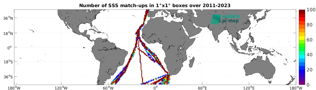
Figure 5: Number of SSS match-ups between TSG (Polarstern) SSS and the SMAP SSS L4 OI v3 - Monthly (ESR) SSS product for the Mid-Low Latitudes 45N-45S Pi-MEP region over 1^\circ \times 1^\circ boxes and for the full satellite product period.
