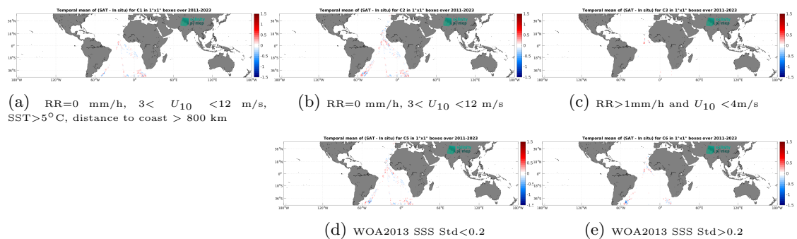
Figure 14: Temporal mean gridded over spatial boxes of size 1^\circ \times 1^\circ of \Delta SSS (SMAP SSS L4 OI v3 - Monthly (ESR) - TSG (Polarstern)) for 5 different subdatasets corresponding to: RR=0 mm/h, 3 < U_{10} < 12 m/s, SST > 5°C, distance to coast > 800 km (a), RR=0 mm/h, 3 < U_{10} < 12 m/s (b), RR > 1mm/h and U_{10} < 4 m/s (c), WOA2013 SSS Std < 0.2 (d), WOA2013 SSS Std > 0.2 (e).
