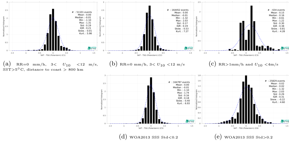
Figure 15: Normalized histogram of \Delta\text{SSS} (SMAP SSS L4 OI v3 - Monthly (ESR) - TSG (Polarstern)) for 5 different subdatasets corresponding to: RR=0 mm/h, 3 < U_{10} < 12 m/s, SST>5°C, distance to coast > 800 km (a), RR=0 mm/h, 3 < U_{10} < 12 m/s (b), RR>1mm/h and U_{10} < 4 m/s (c), WOA2013 SSS Std<0.2 (d), WOA2013 SSS Std>0.2 (e).
