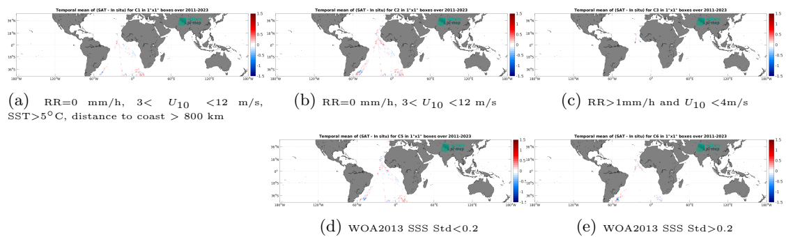
Figure 14: Temporal mean gridded over spatial boxes of size 1^\circ \times 1^\circ of \Delta\text{SSS} (SMAP SSS L4 OI v3 - Monthly (ESR) - TSG (Polarstern)) for 5 different subdatasets corresponding to: RR=0 mm/h, 3 < U_{10} < 12 m/s, SST > 5°C, distance to coast > 800 km (a), RR=0 mm/h, 3 < U_{10} < 12 m/s (b), RR > 1mm/h and U_{10} < 4 m/s (c), WOA2013 SSS Std < 0.2 (d), WOA2013 SSS Std > 0.2 (e).
