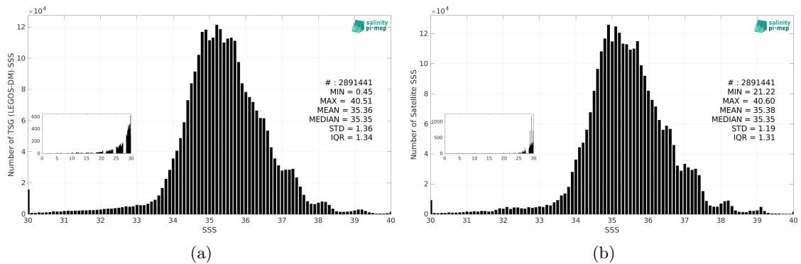
Figure 3: Histograms of SSS from TSG (LEGOS-DM) (a) and SMAP SSS L4 OI v3 - Monthly (ESR) (b) considering all match-up pairs per bins of 0.1 over the Mid-Low Latitudes 45N-45S Pi-MEP region and for the full satellite product period.
