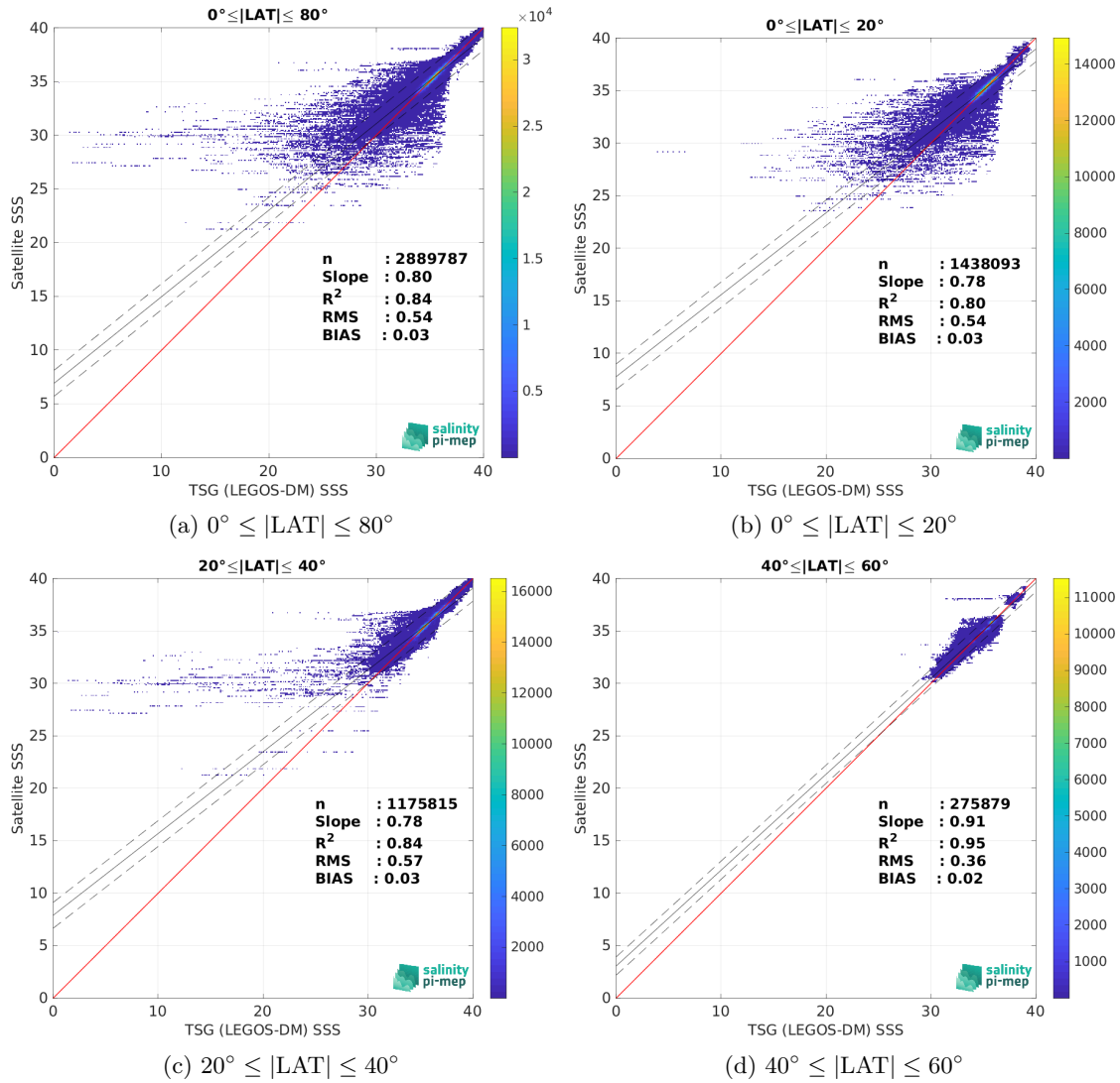
Figure 10: Contour maps of the concentration of SMAP SSS L4 OI v3 - Monthly (ESR) SSS (y-axis) versus TSG (LEGOS-DM) SSS (x-axis) at match-up pairs for different latitude bands. For each plot, the red line shows x=y . The black thin and dashed lines indicate a linear fit through the data cloud and the \pm 95\% confidence levels, respectively. The number match-up pairs n , the slope and R^2 coefficient of the linear fit, the root mean square (RMS) and the mean bias between satellite and in situ data are indicated for each latitude band in each plots.
