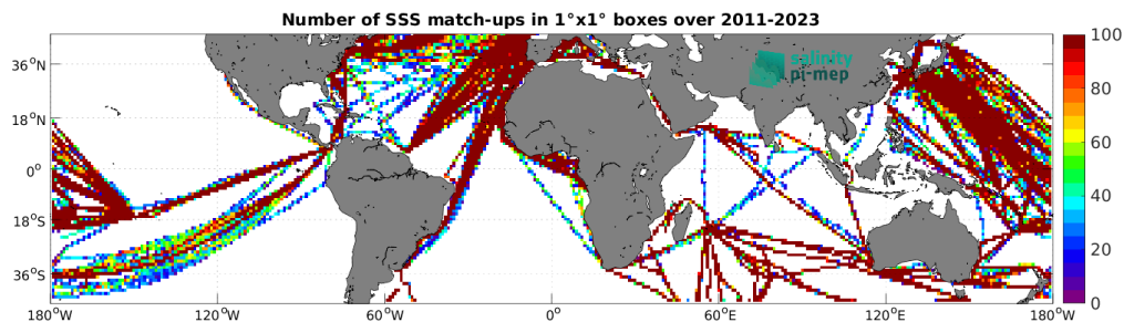
Figure 5: Number of SSS match-ups between TSG (LEGOS-DM) SSS and the SMAP SSS L4 OI v3 - Monthly (ESR) SSS product for the Mid-Low Latitudes 45N-45S Pi-MEP region over 1^\circ \times 1^\circ boxes and for the full satellite product period.
