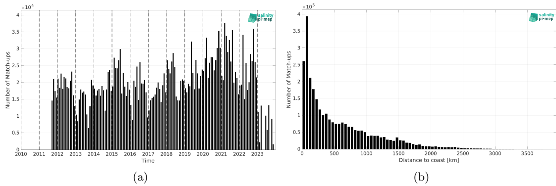
Figure 2: Number of match-ups between TSG (LEGOS-DM) and SMAP SSS L4 OI v3 - Monthly (ESR) SSS as a function of time (a) and as function of the distance to coast (b) over the Mid-Low Latitudes 45N-45S Pi-MEP region and for the full satellite product period.
