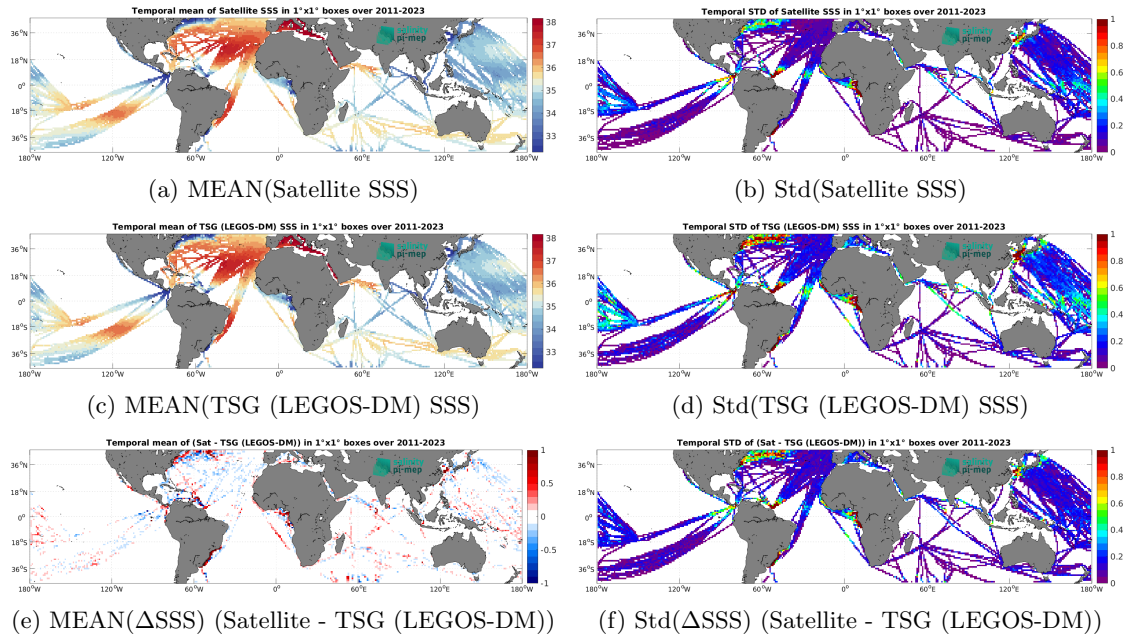
Figure 7: Temporal mean (left) and Std (right) of SSS from SMAP SSS L4 OI v3 - Monthly (ESR) (top), TSG (LEGOS-DM) (middle), and of \Delta SSS (Satellite - TSG (LEGOS-DM)). Only match-up pairs are used to generate these maps.
