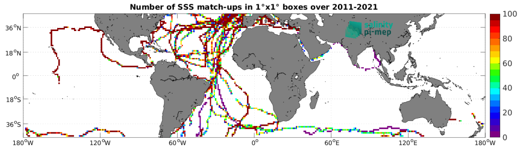
Figure 5: Number of SSS match-ups between TSG (GOSUD-Sailing-ship) SSS and the SMAP SSS L4 OI v3 - Monthly (ESR) SSS product for the Mid-Low Latitudes 45N-45S Pi-MEP region over 1^\circ \times 1^\circ boxes and for the full satellite product period.
