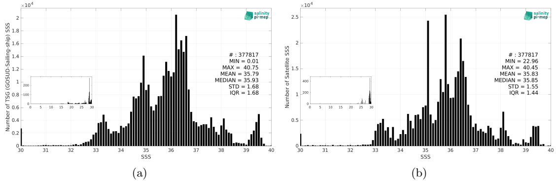
Figure 3: Histograms of SSS from TSG (GOSUD-Sailing-ship) (a) and SMAP SSS L4 OI v3 - Monthly (ESR) (b) considering all match-up pairs per bins of 0.1 over the Mid-Low Latitudes 45N-45S Pi-MEP region and for the full satellite product period.
