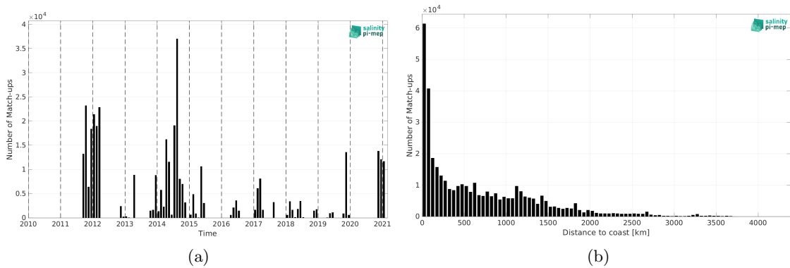
Figure 2: Number of match-ups between TSG (GOSUD-Sailing-ship) and SMAP SSS L4 OI v3 - Monthly (ESR) SSS as a function of time (a) and as function of the distance to coast (b) over the Mid-Low Latitudes 45N-45S Pi-MEP region and for the full satellite product period.
