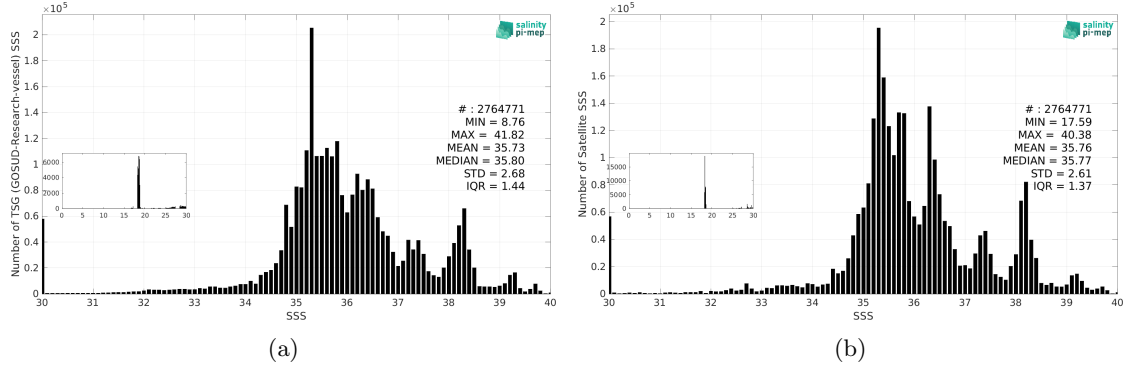
Figure 3: Histograms of SSS from TSG (GOSUD-Research-vessel) (a) and SMAP SSS L4 OI v3 - Monthly (ESR) (b) considering all match-up pairs per bins of 0.1 over the Mid-Low Latitudes 45N-45S Pi-MEP region and for the full satellite product period.
