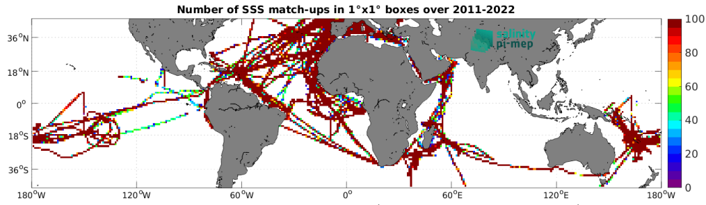
Figure 5: Number of SSS match-ups between TSG (GOSUD-Research-vessel) SSS and the SMAP SSS L4 OI v3 - Monthly (ESR) SSS product for the Mid-Low Latitudes 45N-45S Pi-MEP region over 1^{\circ} \times 1^{\circ} boxes and for the full satellite product period.
