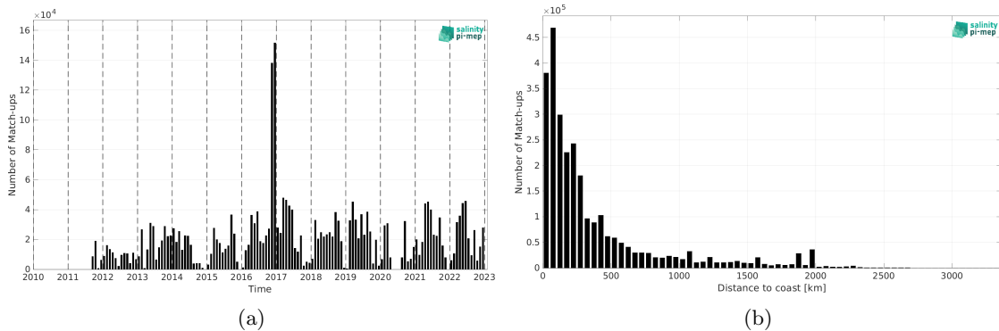
Figure 2: Number of match-ups between TSG (GOSUD-Research-vessel) and SMAP SSS L4 OI v3 - Monthly (ESR) SSS as a function of time (a) and as function of the distance to coast (b) over the Mid-Low Latitudes 45N-45S Pi-MEP region and for the full satellite product period.
