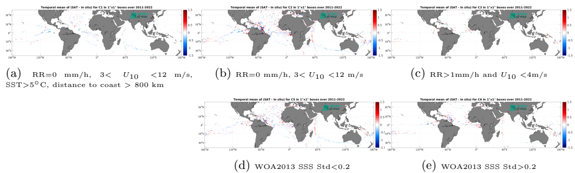
Figure 14: Temporal mean gridded over spatial boxes of size 1^\circ \times 1^\circ of \Delta\text{SSS} (SMAP SSS L4 OI v3 - Monthly (ESR) - TSG (GOSUD-Research-vessel)) for 5 different subdatasets corresponding to: RR=0 mm/h, 3 < U_{10} < 12 m/s, SST > 5°C, distance to coast > 800 km (a), RR=0 mm/h, 3 < U_{10} < 12 m/s (b), RR > 1mm/h and U_{10} < 4 m/s (c), WOA2013 SSS Std < 0.2 (d), WOA2013 SSS Std > 0.2 (e).
