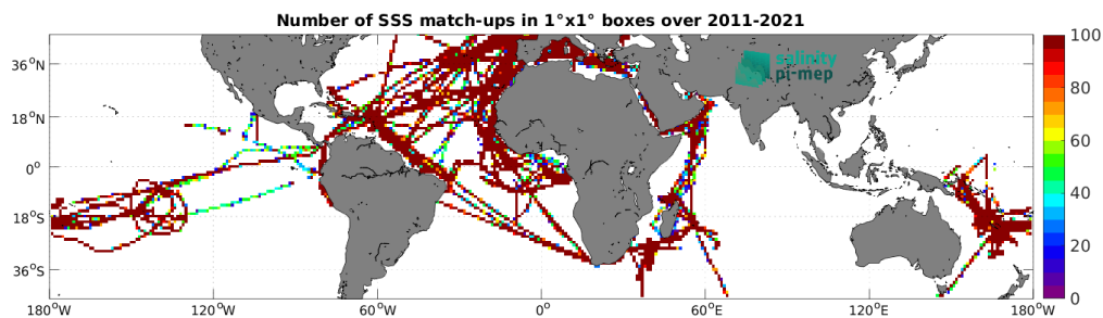
Figure 5: Number of SSS match-ups between TSG (GOSUD-Research-vessel) SSS and the SMAP SSS L4 OI v3 - Monthly (ESR) SSS product for the Mid-Low Latitudes 45N-45S Pi-MEP region over 1^\circ \times 1^\circ boxes and for the full satellite product period.
