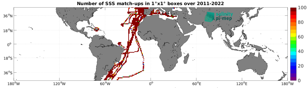
Figure 5: Number of SSS match-ups between TSG (CSIC-UTM) SSS and the SMAP SSS L4 OI v3 - Monthly (ESR) SSS product for the Mid-Low Latitudes 45N-45S Pi-MEP region over 1^\circ \times 1^\circ boxes and for the full satellite product period.
