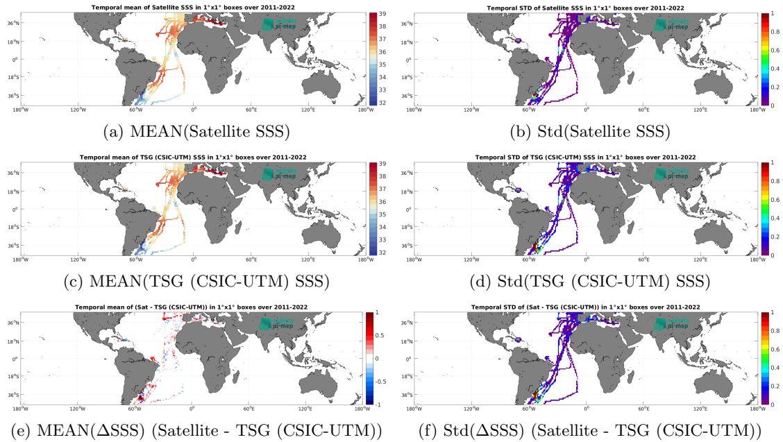
Figure 7: Temporal mean (left) and Std (right) of SSS from SMAP SSS L4 OI v3 - Monthly (ESR) (top), TSG (CSIC-UTM) (middle), and of \Delta SSS (Satellite - TSG (CSIC-UTM)). Only match-up pairs are used to generate these maps.
