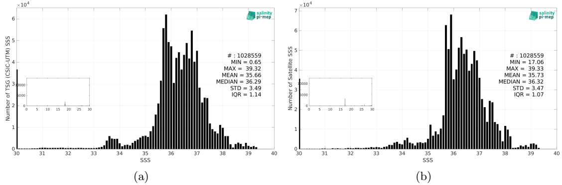
Figure 3: Histograms of SSS from TSG (CSIC-UTM) (a) and SMAP SSS L4 OI v3 - Monthly (ESR) (b) considering all match-up pairs per bins of 0.1 over the Mid-Low Latitudes 45N-45S Pi-MEP region and for the full satellite product period.
