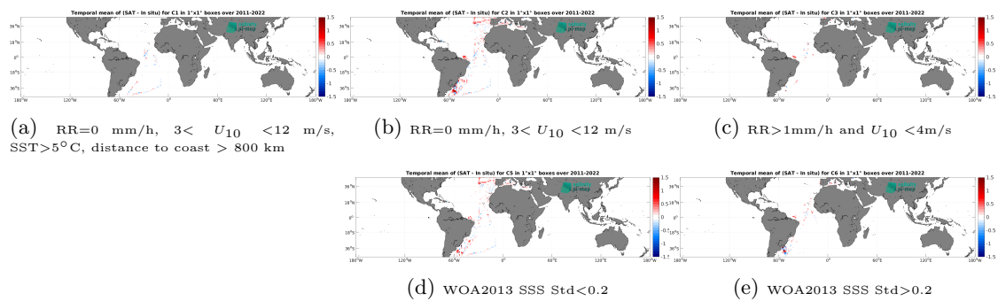
Figure 14: Temporal mean gridded over spatial boxes of size 1^\circ \times 1^\circ of \Delta SSS (SMAP SSS L4 OI v3 - Monthly (ESR) - TSG (CSIC-UTM)) for 5 different subdatasets corresponding to: RR=0 mm/h, 3 < U_{10} < 12 m/s, SST > 5°C, distance to coast > 800 km (a), RR=0 mm/h, 3 < U_{10} < 12 m/s (b), RR > 1mm/h and U_{10} < 4 m/s (c), WOA2013 SSS Std < 0.2 (d), WOA2013 SSS Std > 0.2 (e).
