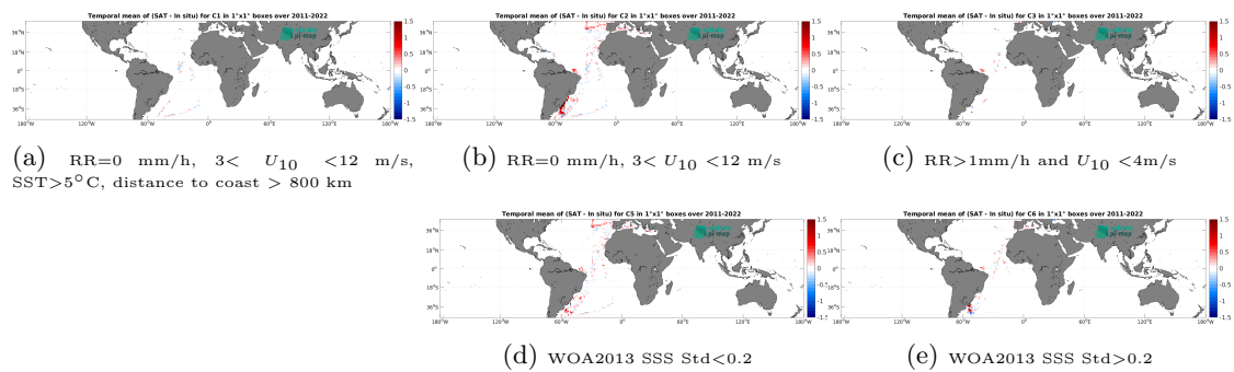
Figure 14: Temporal mean gridded over spatial boxes of size 1^\circ \times 1^\circ of \Delta\text{SSS} (SMAP SSS L4 OI v3 - Monthly (ESR) - TSG (CSIC-UTM)) for 5 different subdatasets corresponding to: RR=0 mm/h, 3 < U_{10} < 12 m/s, SST > 5°C, distance to coast > 800 km (a), RR=0 mm/h, 3 < U_{10} < 12 m/s (b), RR > 1mm/h and U_{10} < 4 m/s (c), WOA2013 SSS Std < 0.2 (d), WOA2013 SSS Std > 0.2 (e).
