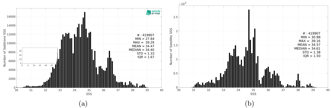
Figure 3: Histograms of SSS from Saildrone (a) and SMAP SSS L4 OI v3 - Monthly (ESR) (b) considering all match-up pairs per bins of 0.1 over the Mid-Low Latitudes 45N-45S Pi-MEP region and for the full satellite product period.
