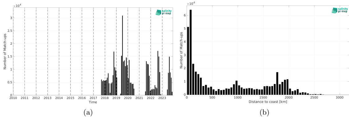
Figure 2: Number of match-ups between Saildrone and SMAP SSS L4 OI v3 - Monthly (ESR) SSS as a function of time (a) and as function of the distance to coast (b) over the Mid-Low Latitudes 45N-45S Pi-MEP region and for the full satellite product period.
