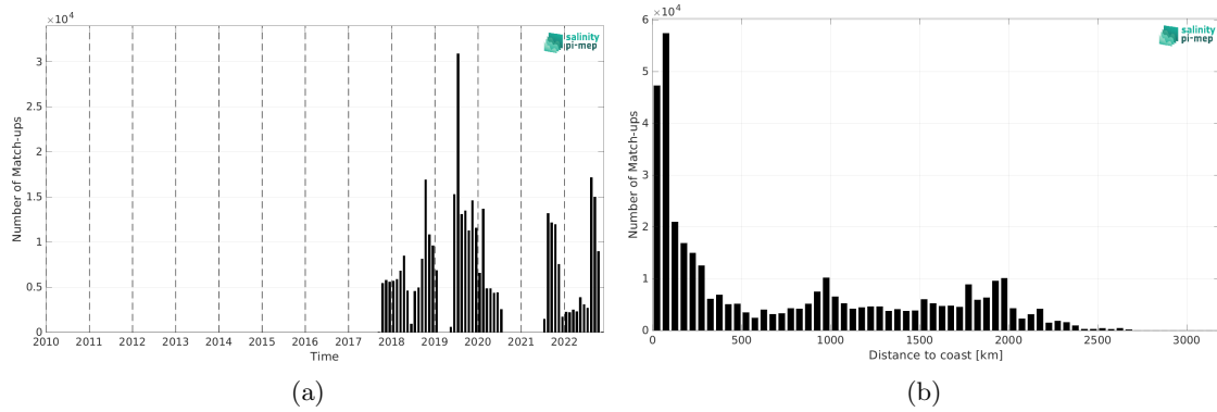
Figure 2: Number of match-ups between Sailldrone and SMAP SSS L4 OI v3 - Monthly (ESR) SSS as a function of time (a) and as function of the distance to coast (b) over the Mid-Low Latitudes 45N-45S Pi-MEP region and for the full satellite product period.
