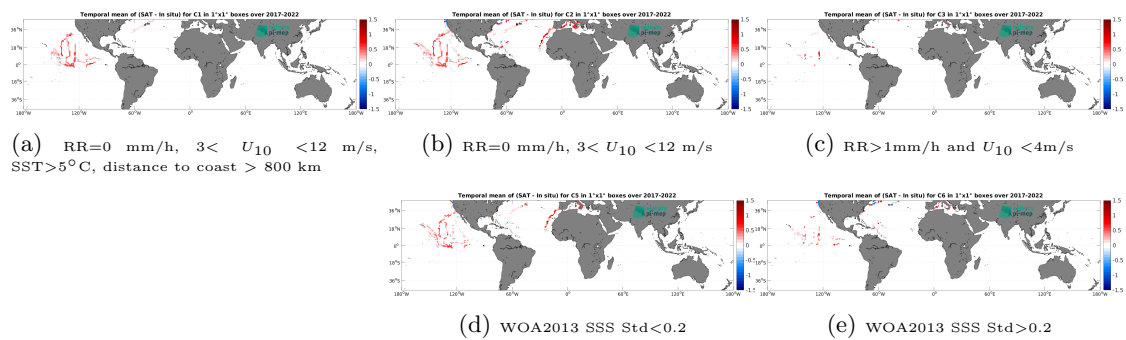
Figure 14: Temporal mean gridded over spatial boxes of size 1^\circ \times 1^\circ of \Delta SSS (SMAP SSS L4 OI v3 - Monthly (ESR) - Sairdrone) for 5 different subdatasets corresponding to:RR=0 mm/h, 3 < U_{10} < 12 m/s, SST >5^\circ\text{C} , distance to coast > 800 km (a), RR=0 mm/h, 3 < U_{10} < 12 m/s (b), RR >1 mm/h and U_{10} < 4 m/s (c), WOA2013 SSS Std <0.2 (d), WOA2013 SSS Std >0.2 (e).
