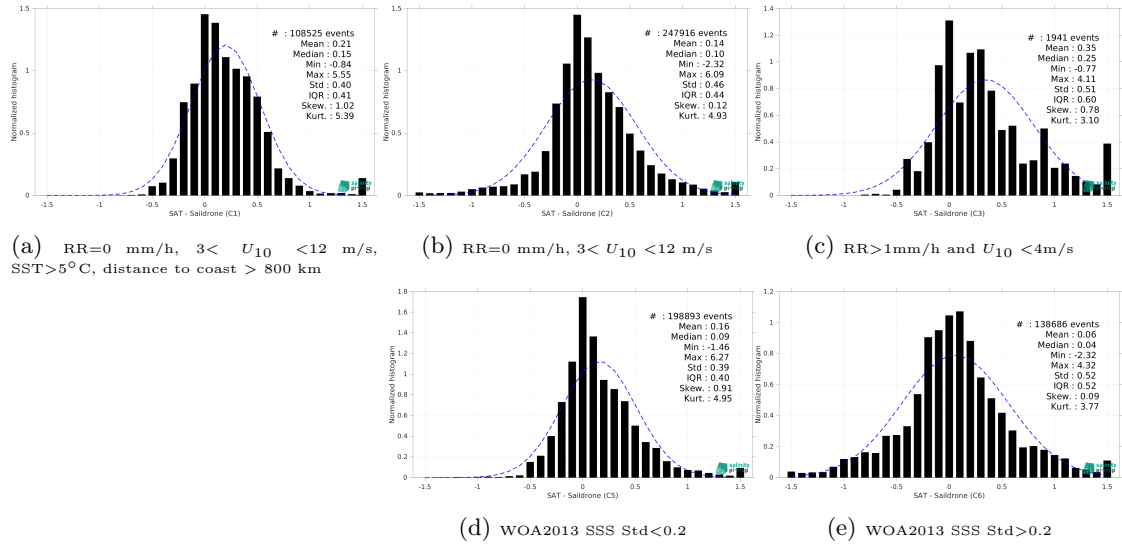
Figure 15: Normalized histogram of \Delta SSS (SMAP SSS L4 OI v3 - Monthly (ESR) - Sairdronne) for 5 different subdatasets corresponding to: RR=0 mm/h, 3 < U_{10} < 12 m/s, SST>5°C, distance to coast > 800 km (a), RR=0 mm/h, 3 < U_{10} < 12 m/s (b), RR>1mm/h and U_{10} < 4 m/s (c), WOA2013 SSS Std<0.2 (d), WOA2013 SSS Std>0.2 (e).
