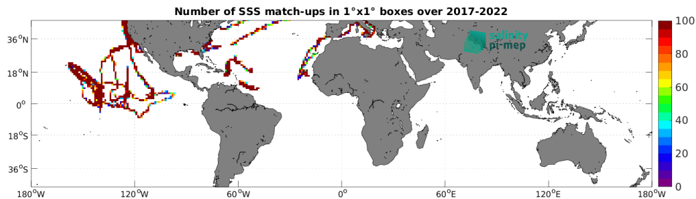
Figure 5: Number of SSS match-ups between Saildrone SSS and the SMAP SSS L4 OI v3 - Monthly (ESR) SSS product for the Mid-Low Latitudes 45N-45S Pi-MEP region over 1^\circ \times 1^\circ boxes and for the full satellite product period.
