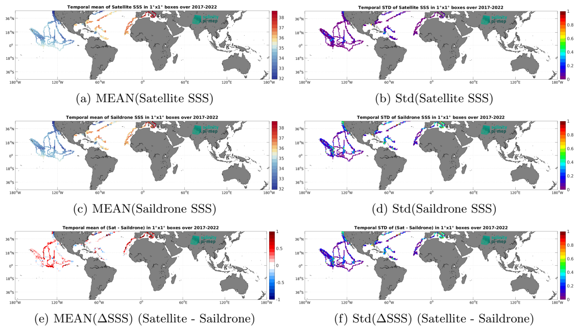
Figure 7: Temporal mean (left) and Std (right) of SSS from SMAP SSS L4 OI v3 - Monthly (ESR) (top), Saildrone (middle), and of \Delta SSS (Satellite - Saildrone). Only match-up pairs are used to generate these maps.
