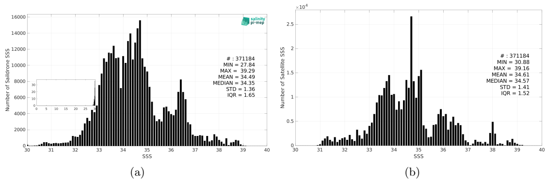
Figure 3: Histograms of SSS from Sailldrone (a) and SMAP SSS L4 OI v3 - Monthly (ESR) (b) considering all match-up pairs per bins of 0.1 over the Mid-Low Latitudes 45N-45S Pi-MEP region and for the full satellite product period.
