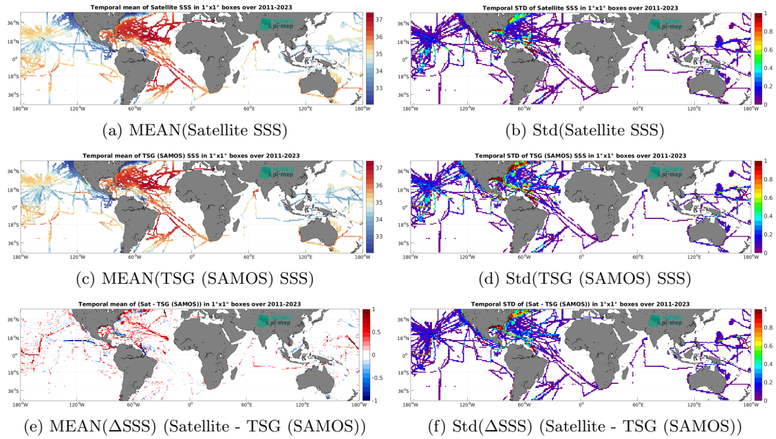
Figure 7: Temporal mean (left) and Std (right) of SSS from SMAP SSS L4 OI v3 - Daily (ESR) (top), TSG (SAMOS) (middle), and of \Delta SSS (Satellite - TSG (SAMOS)). Only match-up pairs are used to generate these maps.
