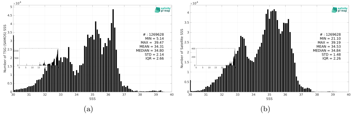
Figure 3: Histograms of SSS from TSG (SAMOS) (a) and SMAP SSS L4 OI v3 - Daily (ESR) (b) considering all match-up pairs per bins of 0.1 over the Mid-Low Latitudes 45N-45S Pi-MEP region and for the full satellite product period.
