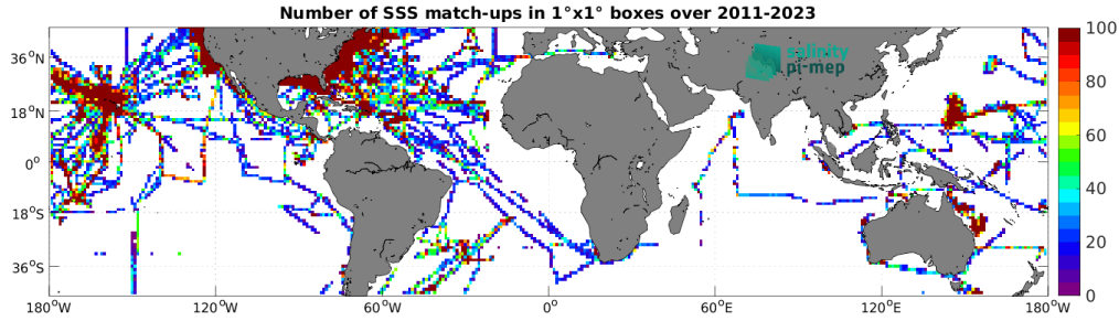
Figure 5: Number of SSS match-ups between TSG (SAMOS) SSS and the SMAP SSS L4 OI v3 - Daily (ESR) SSS product for the Mid-Low Latitudes 45N-45S Pi-MEP region over 1^\circ \times 1^\circ boxes and for the full satellite product period.
