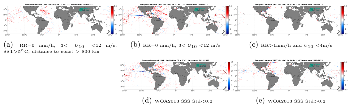
Figure 14: Temporal mean gridded over spatial boxes of size 1^\circ \times 1^\circ of \Delta\text{SSS} (SMAP SSS L4 OI v3 - Daily (ESR) - TSG (SAMOS)) for 5 different subdatasets corresponding to: RR=0 mm/h, 3 < U_{10} < 12 m/s, SST > 5°C, distance to coast > 800 km (a), RR=0 mm/h, 3 < U_{10} < 12 m/s (b), RR > 1mm/h and U_{10} < 4 m/s (c), WOA2013 SSS Std < 0.2 (d), WOA2013 SSS Std > 0.2 (e).
