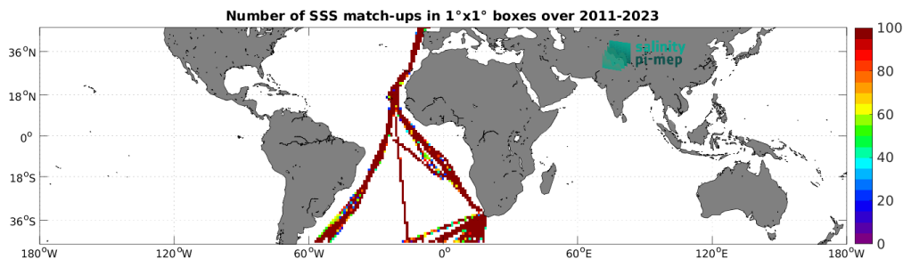
Figure 5: Number of SSS match-ups between TSG (Polarstern) SSS and the SMAP SSS L4 OI v3 - Daily (ESR) SSS product for the Mid-Low Latitudes 45N-45S Pi-MEP region over 1^\circ \times 1^\circ boxes and for the full satellite product period.
