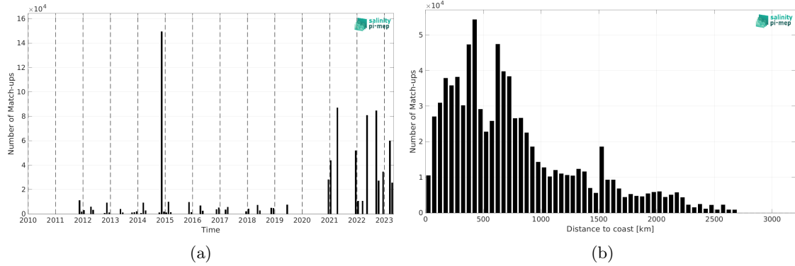
Figure 2: Number of match-ups between TSG (Polarstern) and SMAP SSS L4 OI v3 - Daily (ESR) SSS as a function of time (a) and as function of the distance to coast (b) over the Mid-Low Latitudes 45N-45S Pi-MEP region and for the full satellite product period.
