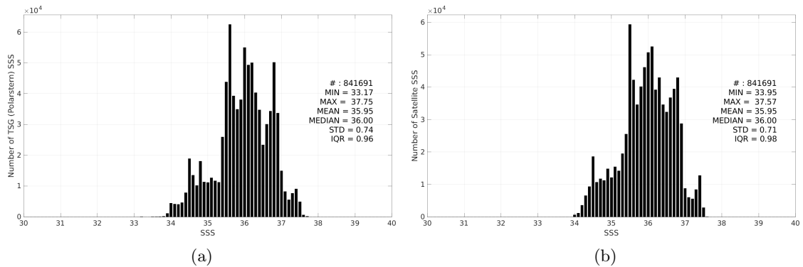
Figure 3: Histograms of SSS from TSG (Polarstern) (a) and SMAP SSS L4 OI v3 - Daily (ESR) (b) considering all match-up pairs per bins of 0.1 over the Mid-Low Latitudes 45N-45S Pi-MEP region and for the full satellite product period.
