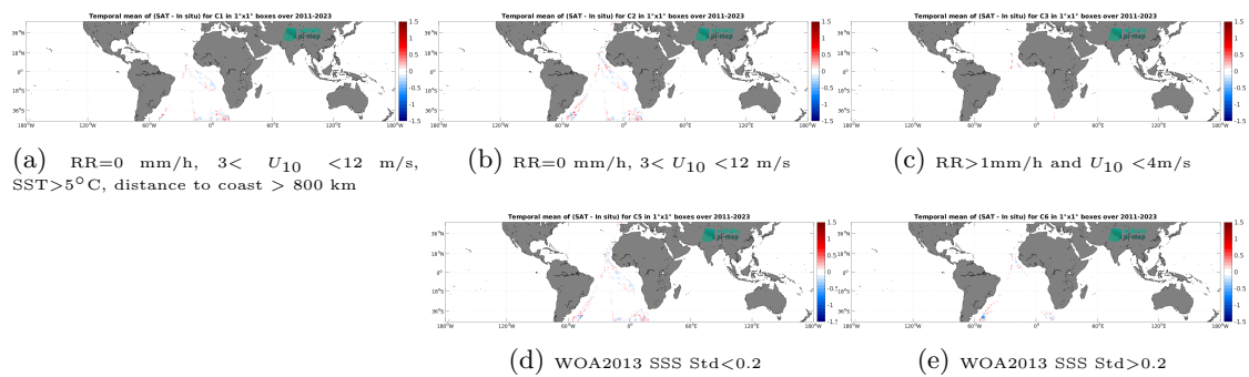
Figure 14: Temporal mean gridded over spatial boxes of size 1^\circ \times 1^\circ of \Delta\text{SSS} (SMAP SSS L4 OI v3 - Daily (ESR) - TSG (Polarstern)) for 5 different subdatasets corresponding to: RR=0 mm/h, 3 < U_{10} < 12 m/s, SST > 5°C, distance to coast > 800 km (a), RR=0 mm/h, 3 < U_{10} < 12 m/s (b), RR > 1mm/h and U_{10} < 4 m/s (c), WOA2013 SSS Std < 0.2 (d), WOA2013 SSS Std > 0.2 (e).
