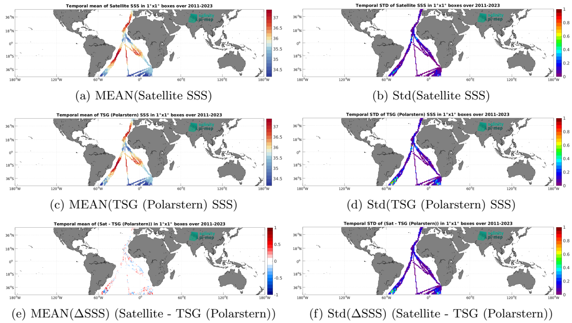
Figure 7: Temporal mean (left) and Std (right) of SSS from SMAP SSS L4 OI v3 - Daily (ESR) (top), TSG (Polarstern) (middle), and of \Delta SSS (Satellite - TSG (Polarstern)). Only match-up pairs are used to generate these maps.
