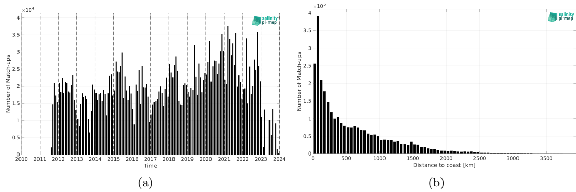
Figure 2: Number of match-ups between TSG (LEGOS-DM) and SMAP SSS L4 OI v3 - Daily (ESR) SSS as a function of time (a) and as function of the distance to coast (b) over the Mid-Low Latitudes 45N-45S Pi-MEP region and for the full satellite product period.
