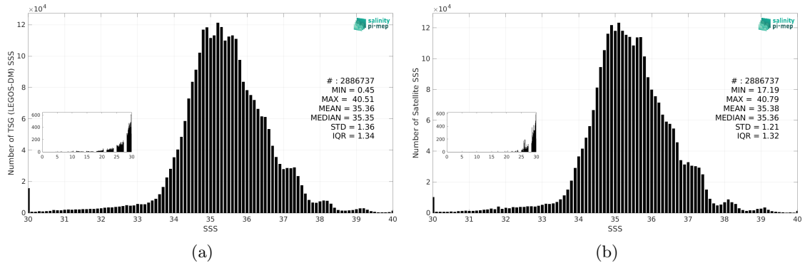
Figure 3: Histograms of SSS from TSG (LEGOS-DM) (a) and SMAP SSS L4 OI v3 - Daily (ESR) (b) considering all match-up pairs per bins of 0.1 over the Mid-Low Latitudes 45N-45S Pi-MEP region and for the full satellite product period.
