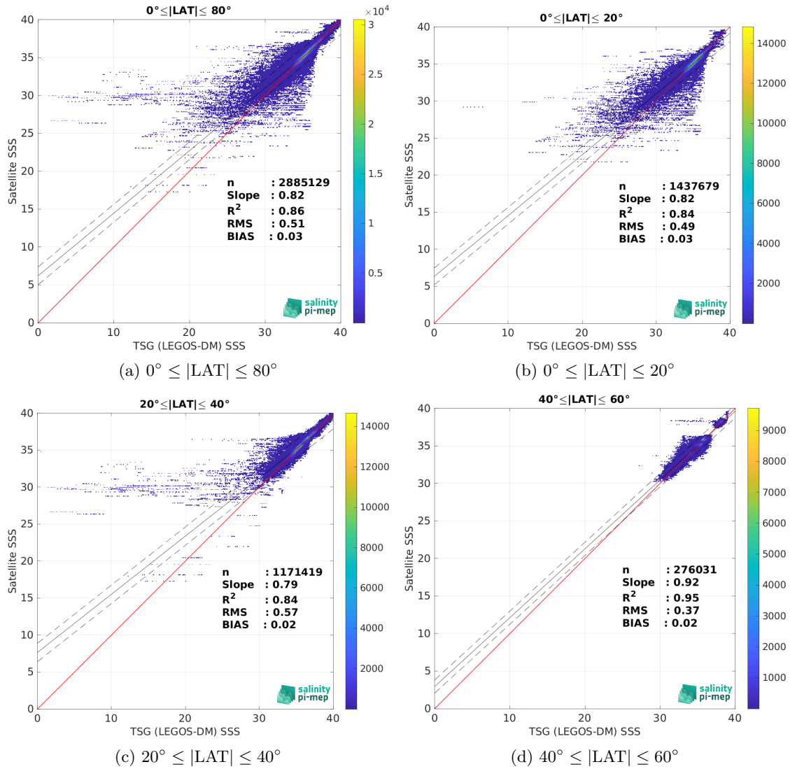
Figure 10: Contour maps of the concentration of SMAP SSS L4 OI v3 - Daily (ESR) SSS (y-axis) versus TSG (LEGOS-DM) SSS (x-axis) at match-up pairs for different latitude bands. For each plot, the red line shows x=y . The black thin and dashed lines indicate a linear fit through the data cloud and the \pm 95\% confidence levels, respectively. The number match-up pairs n , the slope and R^2 coefficient of the linear fit, the root mean square (RMS) and the mean bias between satellite and in situ data are indicated for each latitude band in each plots.
