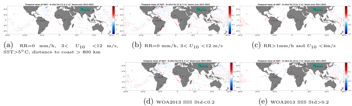
Figure 14: Temporal mean gridded over spatial boxes of size 1^\circ \times 1^\circ of \Delta\text{SSS} (SMAP SSS L4 OI v3 - Daily (ESR) - TSG (LEGOS-DM)) for 5 different subdatasets corresponding to:RR=0 mm/h, 3 < U_{10} < 12 m/s, SST >5^\circ\text{C} , distance to coast > 800 km (a), RR=0 mm/h, 3 < U_{10} < 12 m/s (b), RR >1 mm/h and U_{10} < 4 m/s (c), WOA2013 SSS Std <0.2 (d), WOA2013 SSS Std >0.2 (e).
