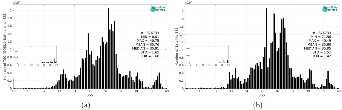
Figure 3: Histograms of SSS from TSG (GOSUD-Sailing-ship) (a) and SMAP SSS L4 OI v3 - Daily (ESR) (b) considering all match-up pairs per bins of 0.1 over the Mid-Low Latitudes 45N-45S Pi-MEP region and for the full satellite product period.
