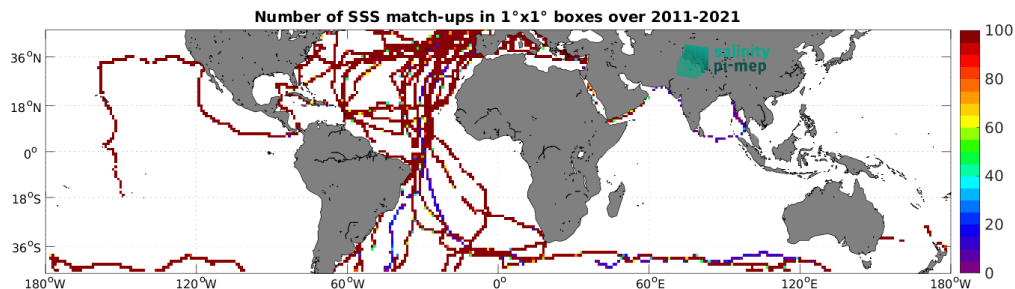
Figure 5: Number of SSS match-ups between TSG (GOSUD-Sailing-ship) SSS and the SMAP SSS L4 OI v3 - Daily (ESR) SSS product for the Mid-Low Latitudes 45N-45S Pi-MEP region over 1^\circ \times 1^\circ boxes and for the full satellite product period.
