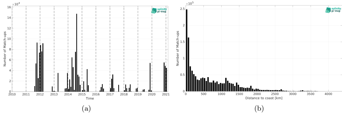
Figure 2: Number of match-ups between TSG (GOSUD-Sailing-ship) and SMAP SSS L4 OI v3 - Daily (ESR) SSS as a function of time (a) and as function of the distance to coast (b) over the Mid-Low Latitudes 45N-45S Pi-MEP region and for the full satellite product period.
