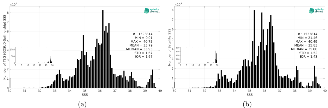
Figure 3: Histograms of SSS from TSG (GOSUD-Sailing-ship) (a) and SMAP SSS L4 OI v3 - Daily (ESR) (b) considering all match-up pairs per bins of 0.1 over the Mid-Low Latitudes 45N-45S Pi-MEP region and for the full satellite product period.
