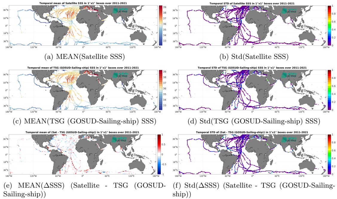
Figure 7: Temporal mean (left) and Std (right) of SSS from SMAP SSS L4 OI v3 - Daily (ESR) (top), TSG (GOSUD-Sailing-ship) (middle), and of \Delta SSS (Satellite - TSG (GOSUD-Sailing-ship)). Only match-up pairs are used to generate these maps.
