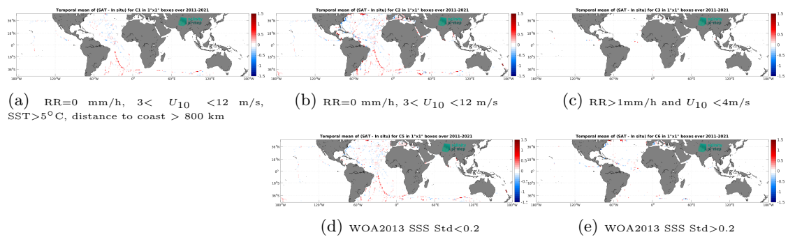
Figure 14: Temporal mean gridded over spatial boxes of size 1^\circ \times 1^\circ of \Delta SSS (SMAP SSS L4 OI v3 - Daily (ESR) - TSG (GOSUD-Sailing-ship)) for 5 different subdatasets corresponding to: RR=0 mm/h, 3 < U_{10} < 12 m/s, SST > 5°C, distance to coast > 800 km (a), RR=0 mm/h, 3 < U_{10} < 12 m/s (b), RR > 1mm/h and U_{10} < 4 m/s (c), WOA2013 SSS Std < 0.2 (d), WOA2013 SSS Std > 0.2 (e).
