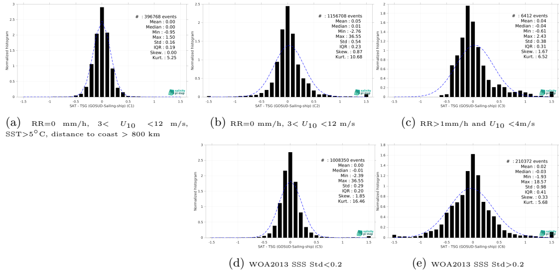
Figure 15: Normalized histogram of \Delta\text{SSS} (SMAP SSS L4 OI v3 - Daily (ESR) - TSG (GOSUD-Sailing-ship)) for 5 different subdatasets corresponding to: RR=0 mm/h, 3 < U_{10} < 12 m/s, SST > 5^{\circ}\text{C} , distance to coast > 800 km (a), RR=0 mm/h, 3 < U_{10} < 12 m/s (b), RR > 1 mm/h and U_{10} < 4 m/s (c), WOA2013 SSS Std < 0.2 (d), WOA2013 SSS Std > 0.2 (e).
