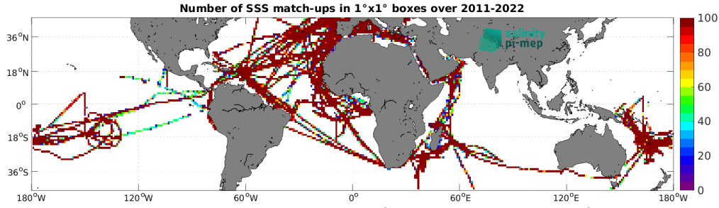
Figure 5: Number of SSS match-ups between TSG (GOSUD-Research-vessel) SSS and the SMAP SSS L4 OI v3 - Daily (ESR) SSS product for the Mid-Low Latitudes 45N-45S Pi-MEP region over 1^\circ \times 1^\circ boxes and for the full satellite product period.
