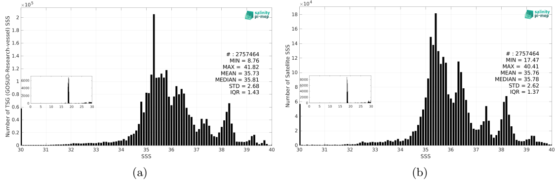
Figure 3: Histograms of SSS from TSG (GOSUD-Research-vessel) (a) and SMAP SSS L4 OI v3 - Daily (ESR) (b) considering all match-up pairs per bins of 0.1 over the Mid-Low Latitudes 45N-45S Pi-MEP region and for the full satellite product period.
