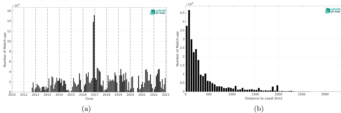
Figure 2: Number of match-ups between TSG (GOSUD-Research-vessel) and SMAP SSS L4 OI v3 - Daily (ESR) SSS as a function of time (a) and as function of the distance to coast (b) over the Mid-Low Latitudes 45N-45S Pi-MEP region and for the full satellite product period.
