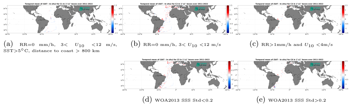
Figure 14: Temporal mean gridded over spatial boxes of size 1^\circ \times 1^\circ of \Delta\text{SSS} (SMAP SSS L4 OI v3 - Daily (ESR) - TSG (CSIC-UTM)) for 5 different subdatasets corresponding to: RR=0 mm/h, 3 < U_{10} < 12 m/s, SST > 5°C, distance to coast > 800 km (a), RR=0 mm/h, 3 < U_{10} < 12 m/s (b), RR > 1mm/h and U_{10} < 4 m/s (c), WOA2013 SSS Std < 0.2 (d), WOA2013 SSS Std > 0.2 (e).
