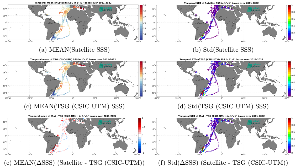
Figure 7: Temporal mean (left) and Std (right) of SSS from SMAP SSS L4 OI v3 - Daily (ESR) (top), TSG (CSIC-UTM) (middle), and of \Delta SSS (Satellite - TSG (CSIC-UTM)). Only match-up pairs are used to generate these maps.
