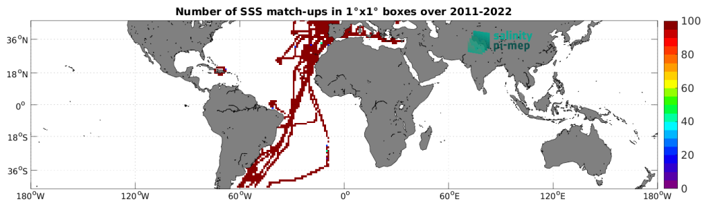
Figure 5: Number of SSS match-ups between TSG (CSIC-UTM) SSS and the SMAP SSS L4 OI v3 - Daily (ESR) SSS product for the Mid-Low Latitudes 45N-45S Pi-MEP region over 1^\circ \times 1^\circ boxes and for the full satellite product period.
