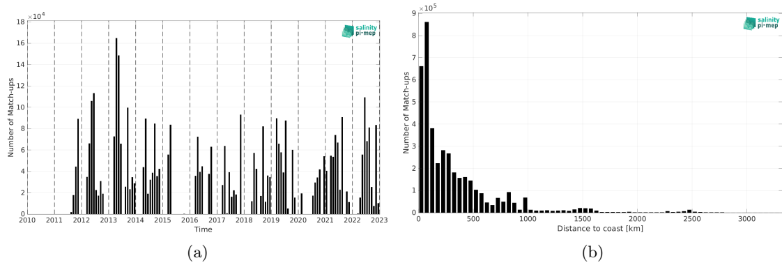
Figure 2: Number of match-ups between TSG (CSIC-UTM) and SMAP SSS L4 OI v3 - Daily (ESR) SSS as a function of time (a) and as function of the distance to coast (b) over the Mid-Low Latitudes 45N-45S Pi-MEP region and for the full satellite product period.
