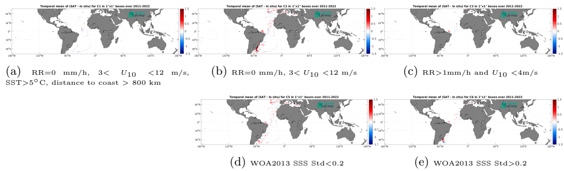
Figure 14: Temporal mean gridded over spatial boxes of size 1^\circ \times 1^\circ of \Delta SSS (SMAP SSS L4 OI v3 - Daily (ESR) - TSG (CSIC-UTM)) for 5 different subdatasets corresponding to: RR=0 mm/h, 3 < U_{10} < 12 m/s, SST > 5°C, distance to coast > 800 km (a), RR=0 mm/h, 3 < U_{10} < 12 m/s (b), RR > 1mm/h and U_{10} < 4 m/s (c), WOA2013 SSS Std < 0.2 (d), WOA2013 SSS Std > 0.2 (e).
