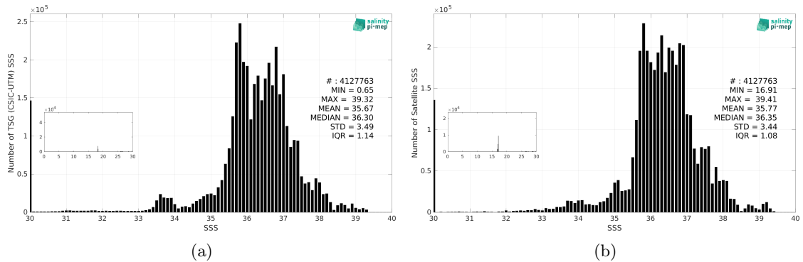
Figure 3: Histograms of SSS from TSG (CSIC-UTM) (a) and SMAP SSS L4 OI v3 - Daily (ESR) (b) considering all match-up pairs per bins of 0.1 over the Mid-Low Latitudes 45N-45S Pi-MEP region and for the full satellite product period.
