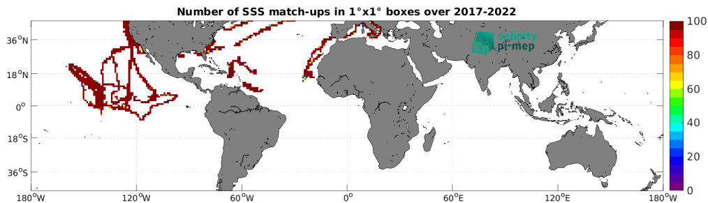
Figure 5: Number of SSS match-ups between Saildrone SSS and the SMAP SSS L4 OI v3 - Daily (ESR) SSS product for the Mid-Low Latitudes 45N-45S Pi-MEP region over 1^\circ \times 1^\circ boxes and for the full satellite product period.
