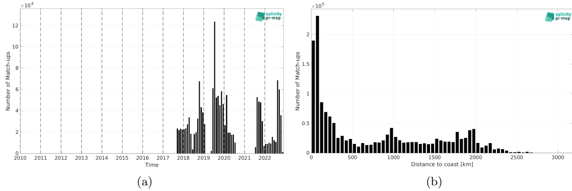
Figure 2: Number of match-ups between Saildrone and SMAP SSS L4 OI v3 - Daily (ESR) SSS as a function of time (a) and as function of the distance to coast (b) over the Mid-Low Latitudes 45N-45S Pi-MEP region and for the full satellite product period.
