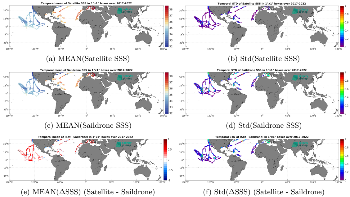
Figure 7: Temporal mean (left) and Std (right) of SSS from SMAP SSS L4 OI v3 - Daily (ESR) (top), Saildrone (middle), and of \Delta SSS (Satellite - Saildrone). Only match-up pairs are used to generate these maps.
