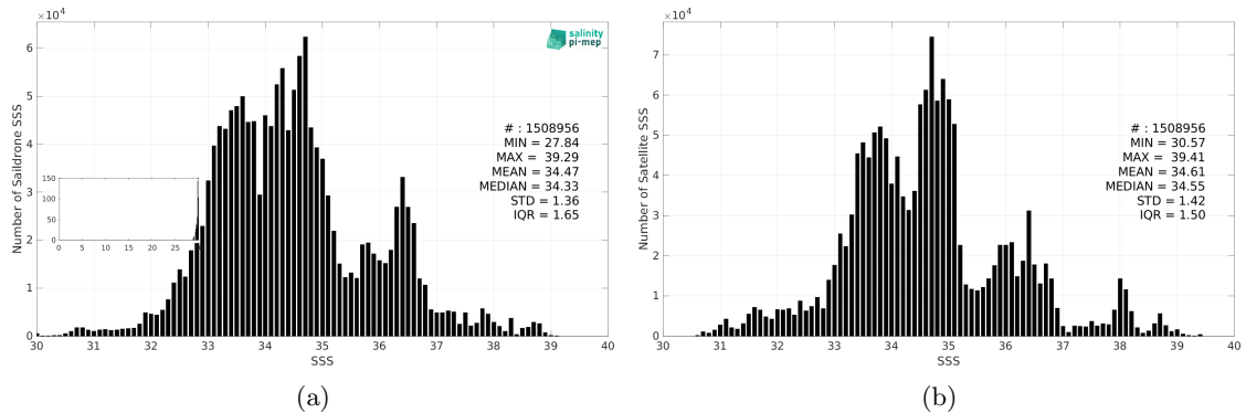
Figure 3: Histograms of SSS from Saildrone (a) and SMAP SSS L4 OI v3 - Daily (ESR) (b) considering all match-up pairs per bins of 0.1 over the Mid-Low Latitudes 45N-45S Pi-MEP region and for the full satellite product period.
