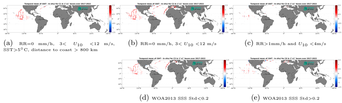
Figure 14: Temporal mean gridded over spatial boxes of size 1^\circ \times 1^\circ of \Delta SSS (SMAP SSS L4 OI v3 - Daily (ESR) - Saildrone) for 5 different subdatasets corresponding to: RR=0 mm/h, 3 < U_{10} < 12 m/s, SST > 5°C, distance to coast > 800 km (a), RR=0 mm/h, 3 < U_{10} < 12 m/s (b), RR > 1mm/h and U_{10} < 4 m/s (c), WOA2013 SSS Std < 0.2 (d), WOA2013 SSS Std > 0.2 (e).
