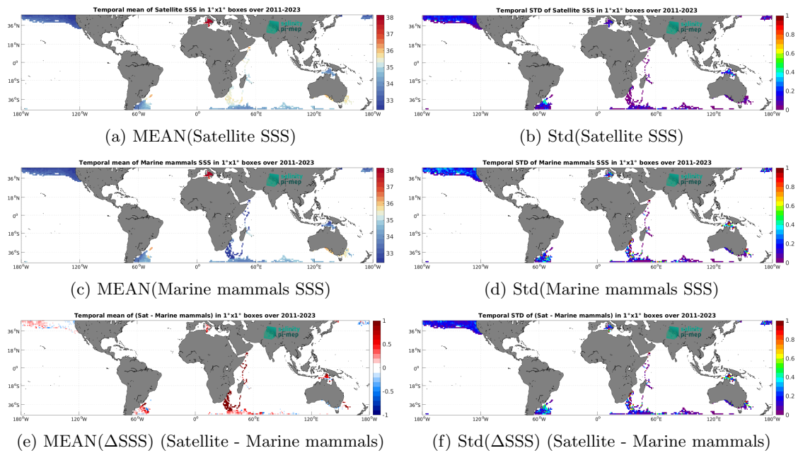
Figure 7: Temporal mean (left) and Std (right) of SSS from SMAP SSS L4 OI v3 - Daily (ESR) (top), Marine mammals (middle), and of \Delta SSS (Satellite - Marine mammals). Only match-up pairs are used to generate these maps.
