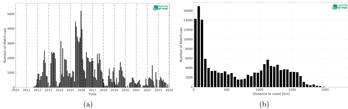
Figure 2: Number of match-ups between Marine mammals and SMAP SSS L4 OI v3 - Daily (ESR) SSS as a function of time (a) and as function of the distance to coast (b) over the Mid-Low Latitudes 45N-45S Pi-MEP region and for the full satellite product period.
