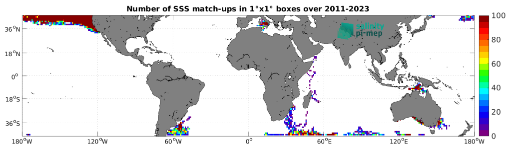
Figure 5: Number of SSS match-ups between Marine mammals SSS and the SMAP SSS L4 OI v3 - Daily (ESR) SSS product for the Mid-Low Latitudes 45N-45S Pi-MEP region over 1^\circ \times 1^\circ boxes and for the full satellite product period.
