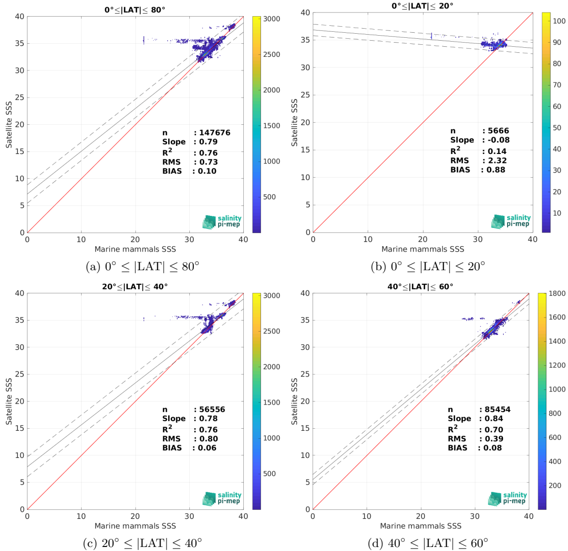
Figure 10: Contour maps of the concentration of SMAP SSS L4 OI v3 - Daily (ESR) SSS (y-axis) versus Marine mammals SSS (x-axis) at match-up pairs for different latitude bands. For each plot, the red line shows x=y . The black thin and dashed lines indicate a linear fit through the data cloud and the \pm 95\% confidence levels, respectively. The number match-up pairs n , the slope and R^2 coefficient of the linear fit, the root mean square (RMS) and the mean bias between satellite and in situ data are indicated for each latitude band in each plots.
