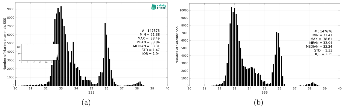
Figure 3: Histograms of SSS from Marine mammals (a) and SMAP SSS L4 OI v3 - Daily (ESR) (b) considering all match-up pairs per bins of 0.1 over the Mid-Low Latitudes 45N-45S Pi-MEP region and for the full satellite product period.
