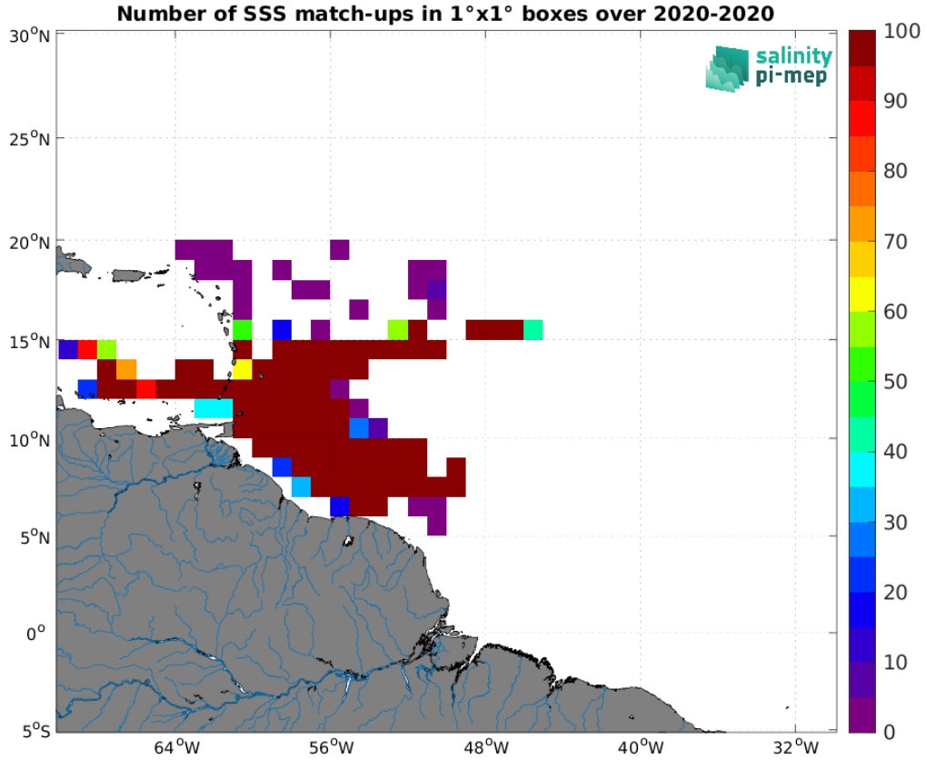
Figure 5: Number of SSS match-ups between EUREC4A SSS and the SMAP SSS L4 OI v3 - Daily (ESR) SSS product for the Mid-Low Latitudes 45N-45S Pi-MEP region over 1^\circ \times 1^\circ boxes and for the full satellite product period.
