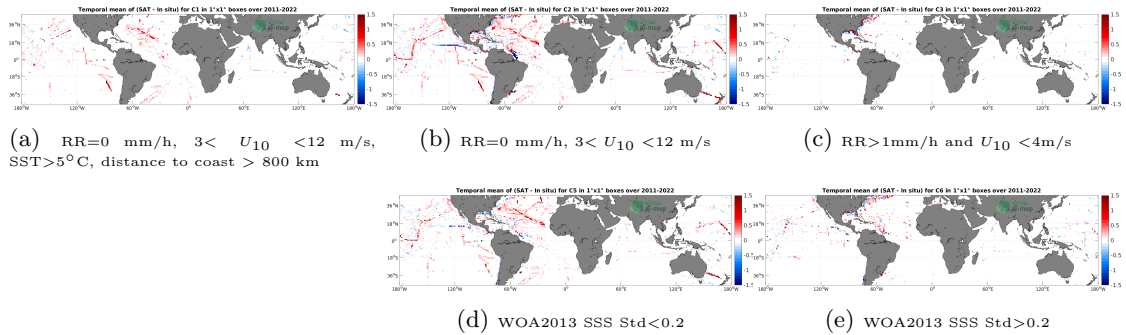
Figure 12: Temporal mean gridded over spatial boxes of size 1^\circ \times 1^\circ of \Delta SSS (SMAP SSS L4 OI v2 - 7 Days (ESR) - TSG (SAMOS)) for 5 different subdatasets corresponding to: RR=0 mm/h, 3 < U_{10} < 12 m/s, SST>5°C, distance to coast > 800 km (a), RR=0 mm/h, 3 < U_{10} < 12 m/s (b), RR>1mm/h and U_{10} < 4 m/s (c), WOA2013 SSS Std<0.2 (d), WOA2013 SSS Std>0.2 (e).
