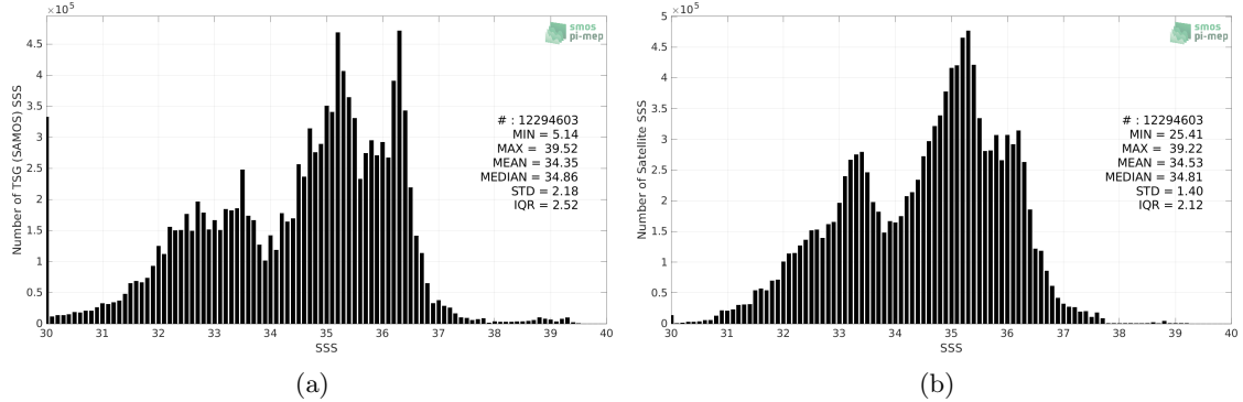
Figure 2: Histograms of SSS from TSG (SAMOS) (a) and SMAP SSS L4 OI v2 - 7 Days (ESR) (b) considering all match-up pairs per bins of 0.1 over the Mid-Low Latitudes 45N-45S Pi-MEP region and for the full satellite product period.
