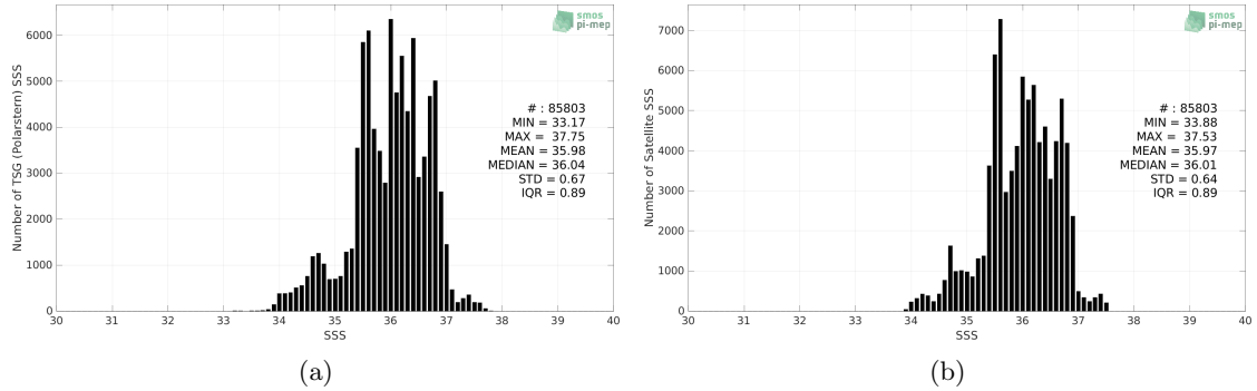
Figure 2: Histograms of SSS from TSG (Polarstern) (a) and SMAP SSS L4 OI v2 - 7 Days (ESR) (b) considering all match-up pairs per bins of 0.1 over the Mid-Low Latitudes 45N-45S Pi-MEP region and for the full satellite product period.
