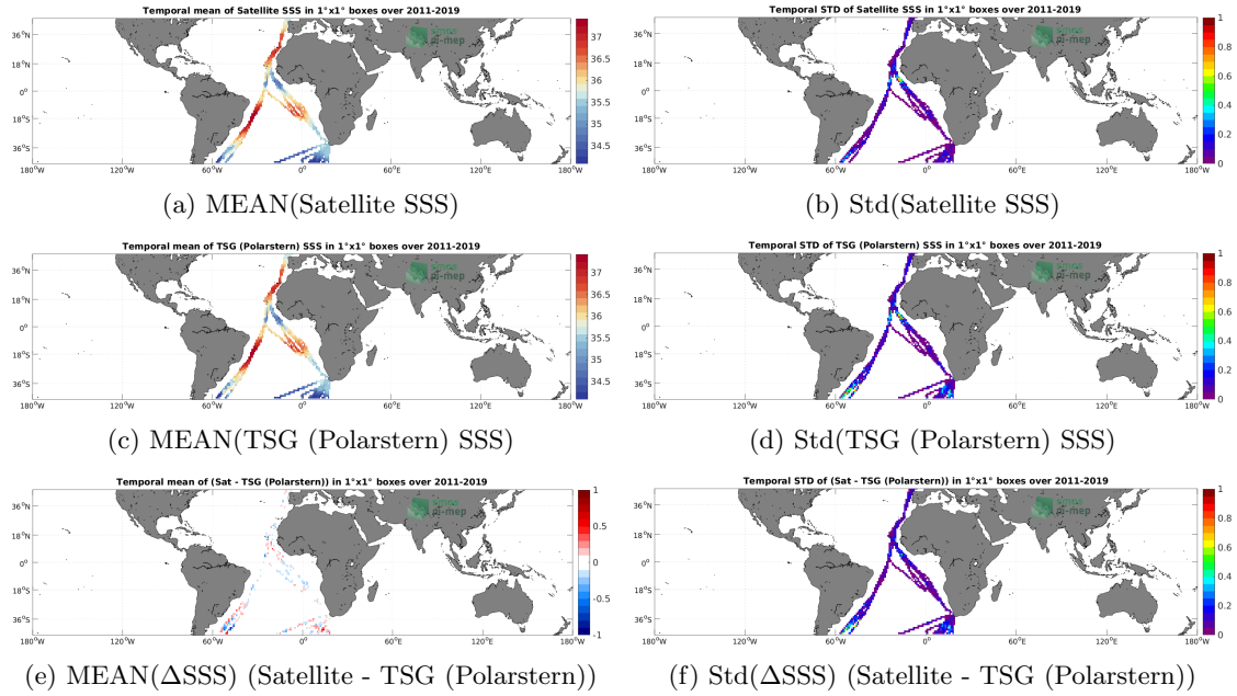
Figure 6: Temporal mean (left) and Std (right) of SSS from SMAP SSS L4 OI v2 - 7 Days (ESR) (top), TSG (Polarstern) (middle), and of \Delta SSS (Satellite - TSG (Polarstern)). Only match-up pairs are used to generate these maps.
