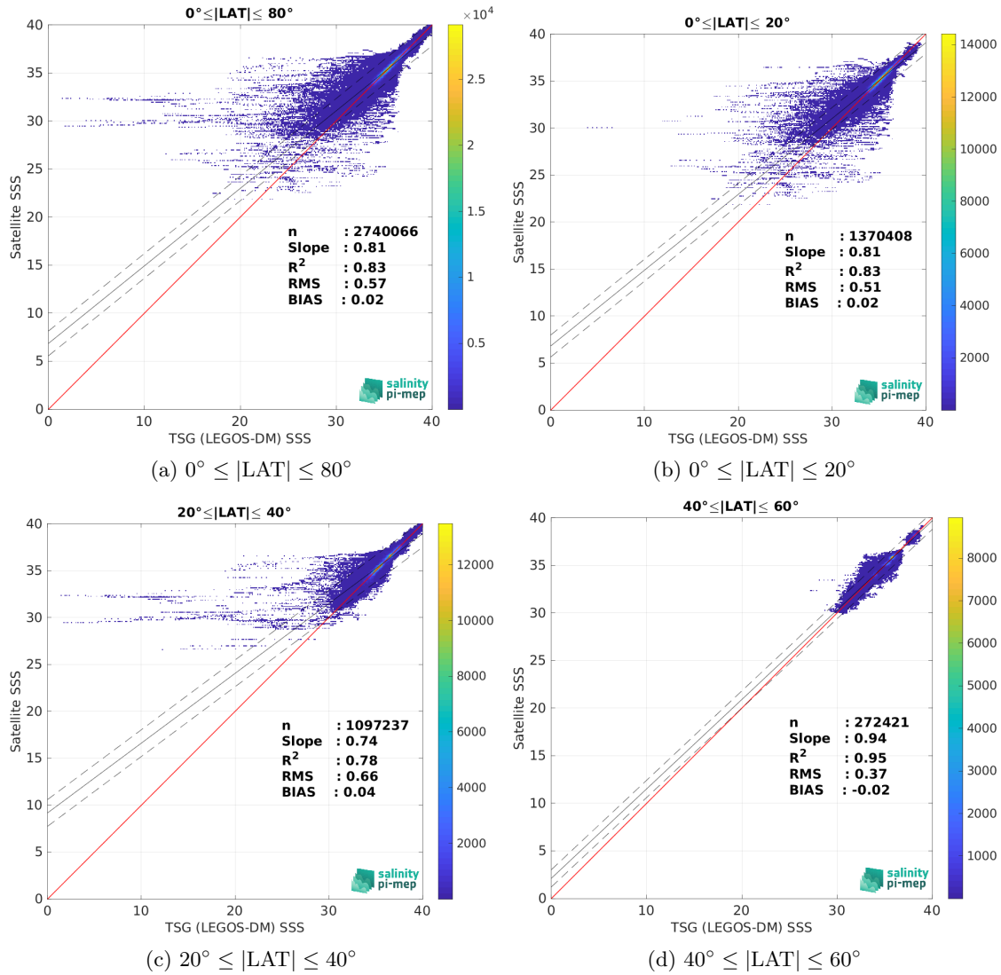
Figure 9: Contour maps of the concentration of SMAP SSS L4 OI v2 - 7 Days (ESR) SSS (y-axis) versus TSG (LEGOS-DM) SSS (x-axis) at match-up pairs for different latitude bands. For each plot, the red line shows x=y . The black thin and dashed lines indicate a linear fit through the data cloud and the \pm 95\% confidence levels, respectively. The number match-up pairs n , the slope and R^2 coefficient of the linear fit, the root mean square (RMS) and the mean bias between satellite and in situ data are indicated for each latitude band in each plots.
