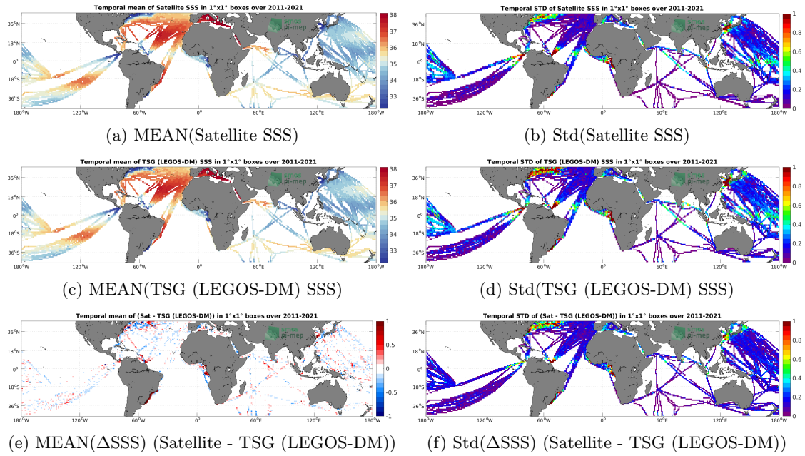
Figure 6: Temporal mean (left) and Std (right) of SSS from SMAP SSS L4 OI v2 - 7 Days (ESR) (top), TSG (LEGOS-DM) (middle), and of \Delta SSS (Satellite - TSG (LEGOS-DM)). Only match-up pairs are used to generate these maps.
