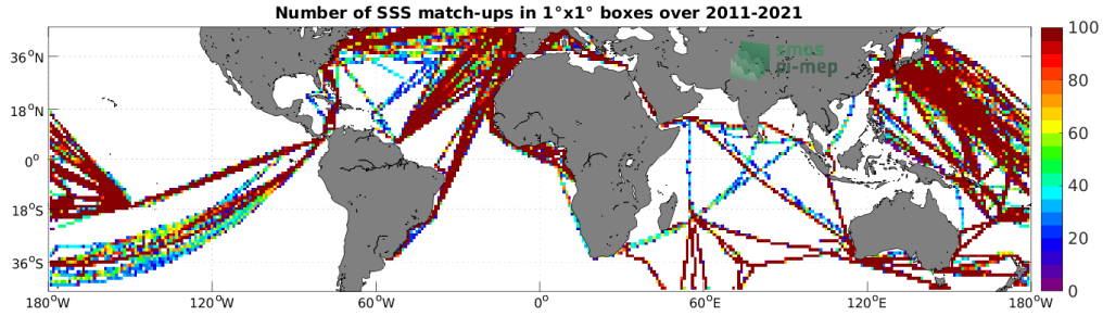
Figure 4: Number of SSS match-ups between TSG (LEGOS-DM) SSS and the SMAP SSS L4 OI v2 - 7 Days (ESR) SSS product for the Mid-Low Latitudes 45N-45S Pi-MEP region over 1^\circ \times 1^\circ boxes and for the full satellite product period.
