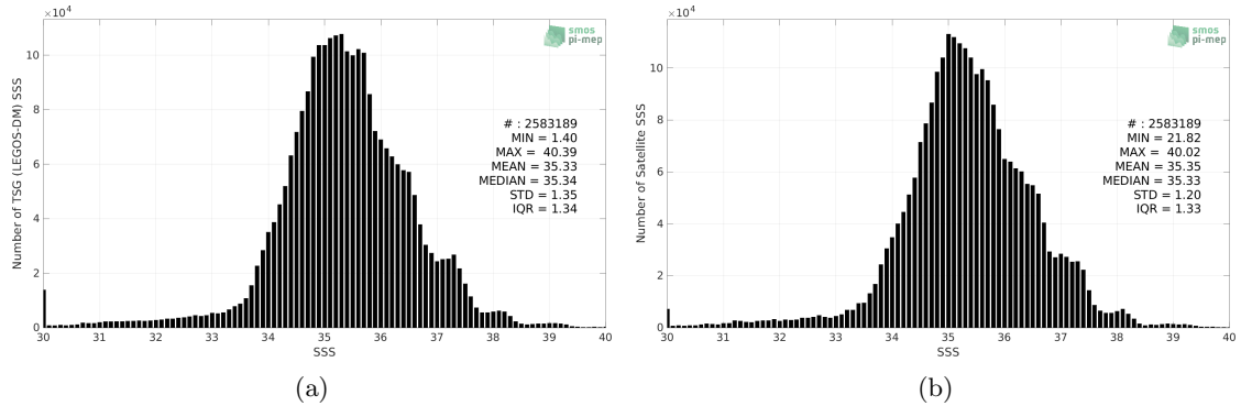
Figure 2: Histograms of SSS from TSG (LEGOS-DM) (a) and SMAP SSS L4 OI v2 - 7 Days (ESR) (b) considering all match-up pairs per bins of 0.1 over the Mid-Low Latitudes 45N-45S Pi-MEP region and for the full satellite product period.
