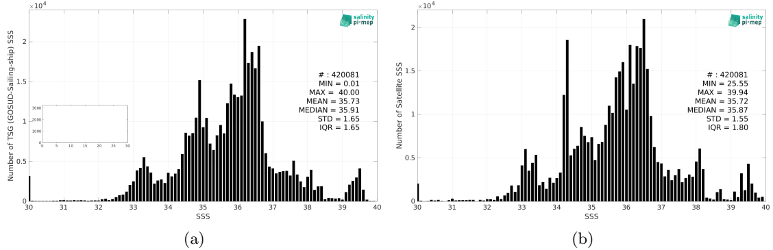
Figure 2: Histograms of SSS from TSG (GOSUD-Sailing-ship) (a) and SMAP SSS L4 OI v2 - 7 Days (ESR) (b) considering all match-up pairs per bins of 0.1 over the Mid-Low Latitudes 45N-45S Pi-MEP region and for the full satellite product period.
