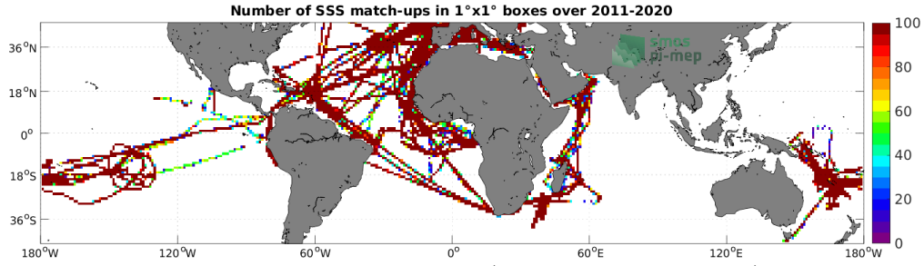
Figure 4: Number of SSS match-ups between TSG (GOSUD-Research-vessel) SSS and the SMAP SSS L4 OI v2 - 7 Days (ESR) SSS product for the Mid-Low Latitudes 45N-45S Pi-MEP region over 1^\circ \times 1^\circ boxes and for the full satellite product period.
