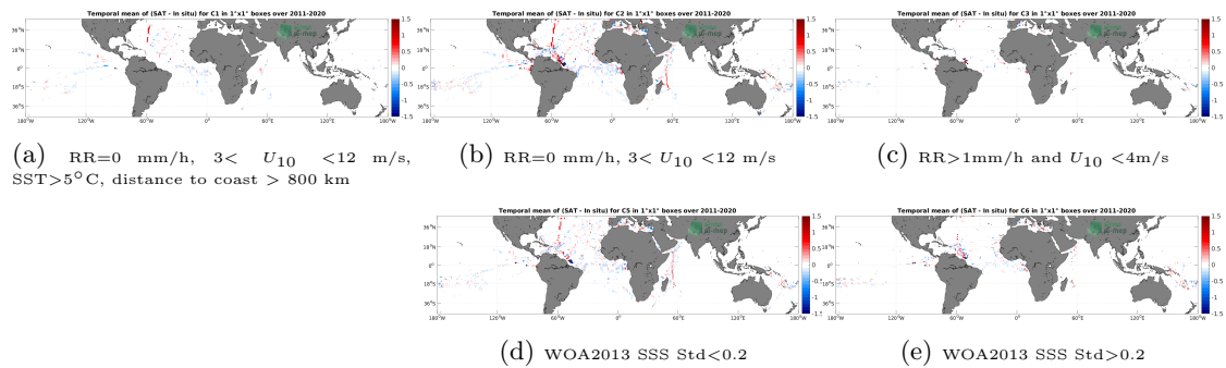
Figure 12: Temporal mean gridded over spatial boxes of size 1^\circ \times 1^\circ of \Delta SSS (SMAP SSS L4 OI v2 - 7 Days (ESR) - TSG (GOSUD-Research-vessel)) for 5 different subdatasets corresponding to: RR=0 mm/h, 3 < U_{10} < 12 m/s, SST > 5°C, distance to coast > 800 km (a), RR=0 mm/h, 3 < U_{10} < 12 m/s (b), RR > 1mm/h and U_{10} < 4 m/s (c), WOA2013 SSS Std < 0.2 (d), WOA2013 SSS Std > 0.2 (e).
