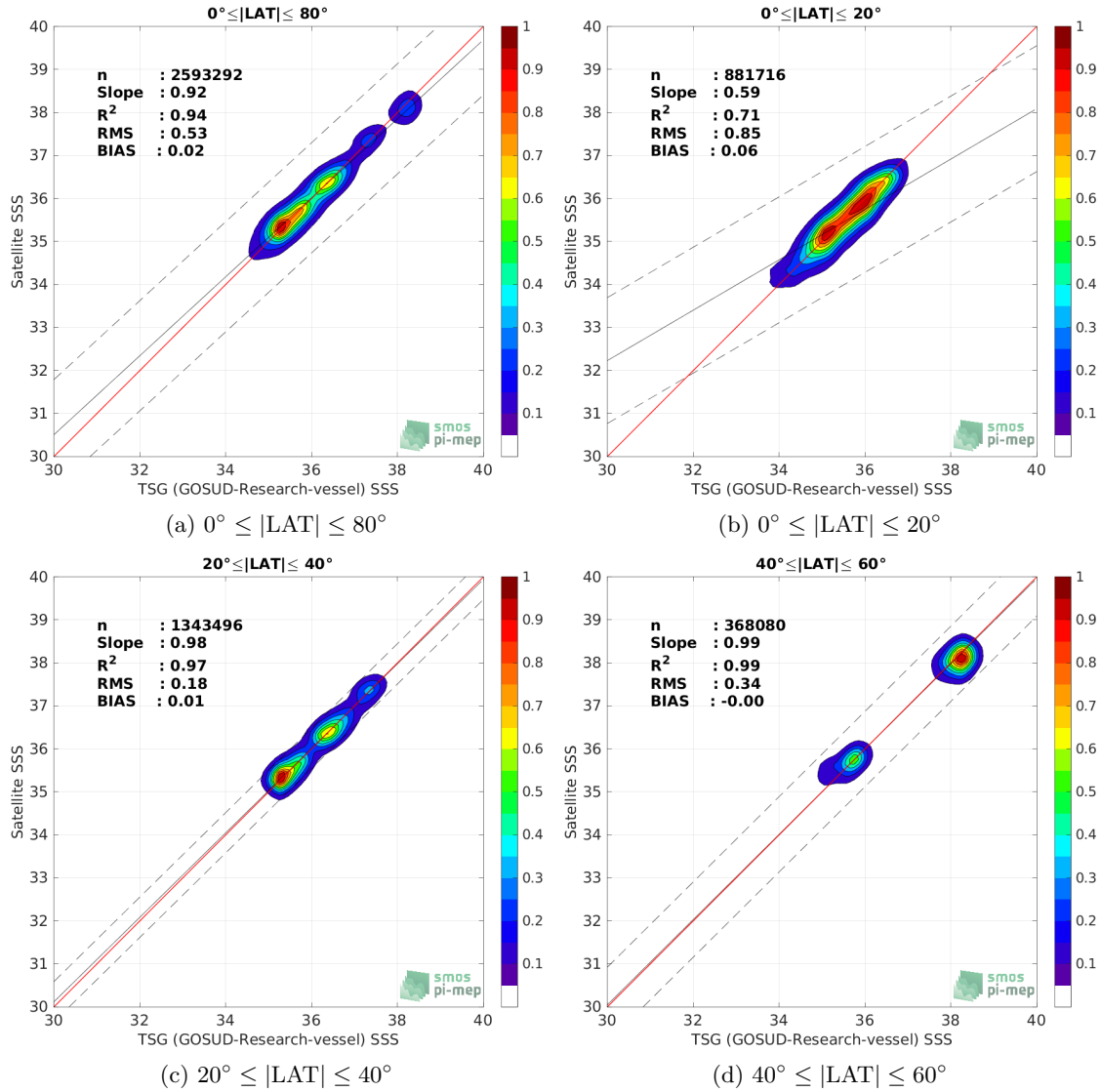
Figure 9: Contour maps of the concentration of SMAP SSS L4 OI v2 - 7 Days (ESR) SSS (y-axis) versus TSG (GOSUD-Research-vessel) SSS (x-axis) at match-up pairs for different latitude bands. For each plot, the red line shows x=y . The black thin and dashed lines indicate a linear fit through the data cloud and the \pm 95\% confidence levels, respectively. The number match-up pairs n , the slope and R^2 coefficient of the linear fit, the root mean square (RMS) and the mean bias between satellite and in situ data are indicated for each latitude band in each plots.
