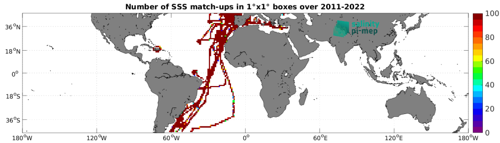
Figure 4: Number of SSS match-ups between TSG (CSIC-UTM) SSS and the SMAP SSS L4 OI v2 - 7 Days (ESR) SSS product for the Mid-Low Latitudes 45N-45S Pi-MEP region over 1^\circ \times 1^\circ boxes and for the full satellite product period.
