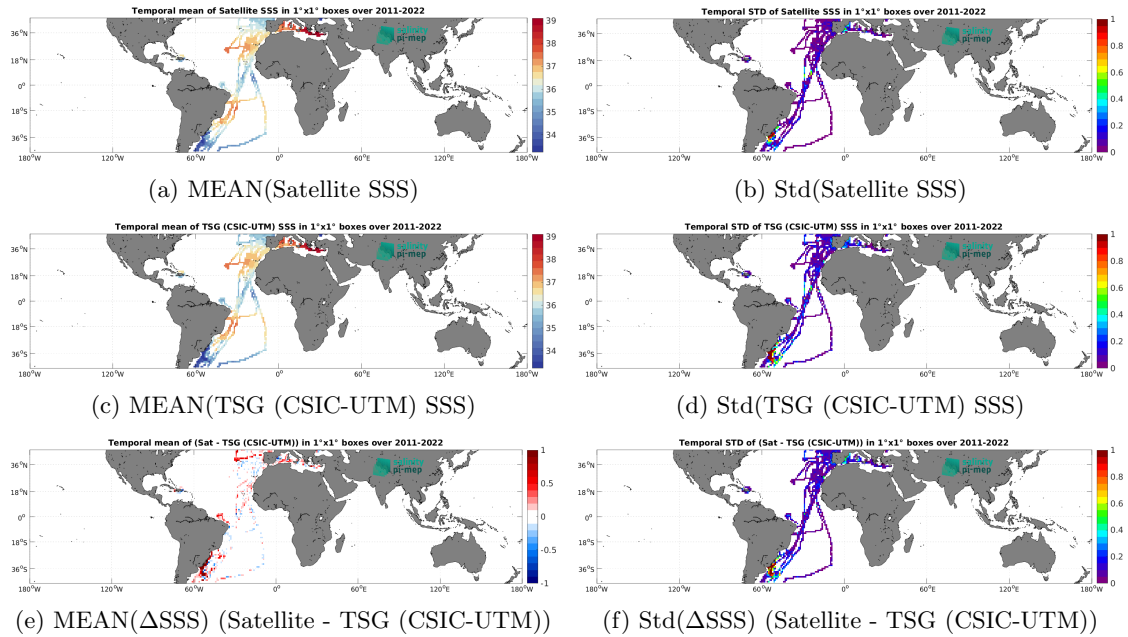
Figure 6: Temporal mean (left) and Std (right) of SSS from SMAP SSS L4 OI v2 - 7 Days (ESR) (top), TSG (CSIC-UTM) (middle), and of \Delta SSS (Satellite - TSG (CSIC-UTM)). Only match-up pairs are used to generate these maps.
