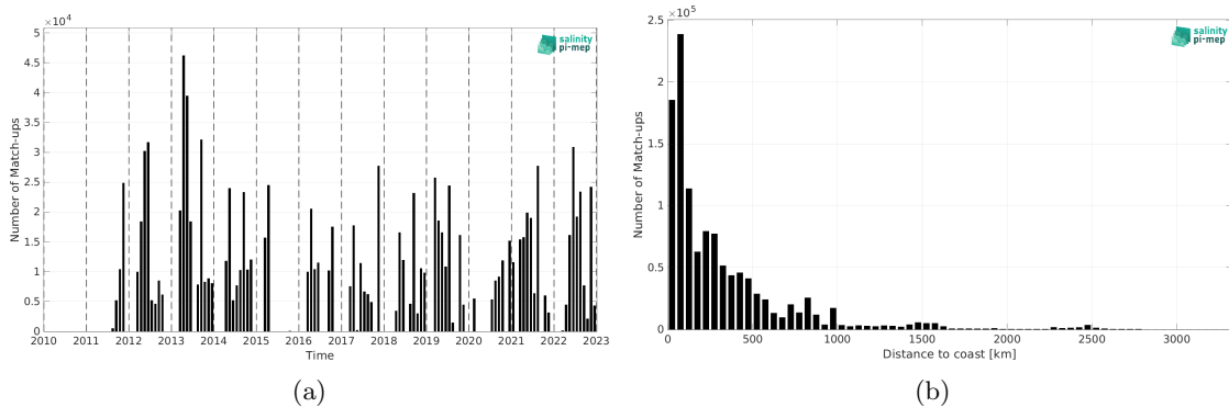
Figure 1: Number of match-ups between TSG (CSIC-UTM) and SMAP SSS L4 OI v2 - 7 Days (ESR) SSS as a function of time (a) and as function of the distance to coast (b) over the Mid-Low Latitudes 45N-45S Pi-MEP region and for the full satellite product period.
