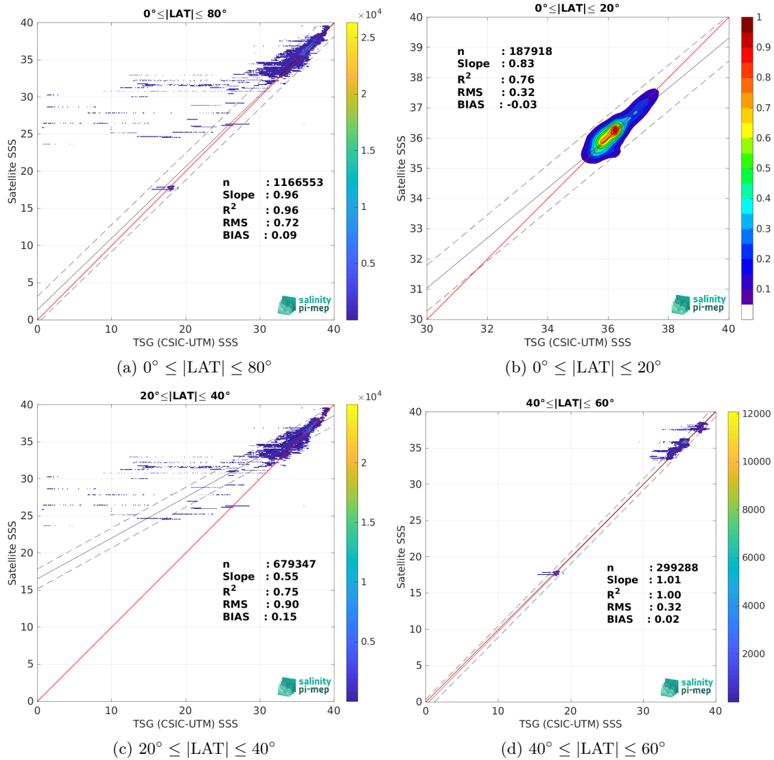
Figure 9: Contour maps of the concentration of SMAP SSS L4 OI v2 - 7 Days (ESR) SSS (y-axis) versus TSG (CSIC-UTM) SSS (x-axis) at match-up pairs for different latitude bands. For each plot, the red line shows x=y . The black thin and dashed lines indicate a linear fit through the data cloud and the \pm 95\% confidence levels, respectively. The number match-up pairs n , the slope and R^2 coefficient of the linear fit, the root mean square (RMS) and the mean bias between satellite and in situ data are indicated for each latitude band in each plots.
