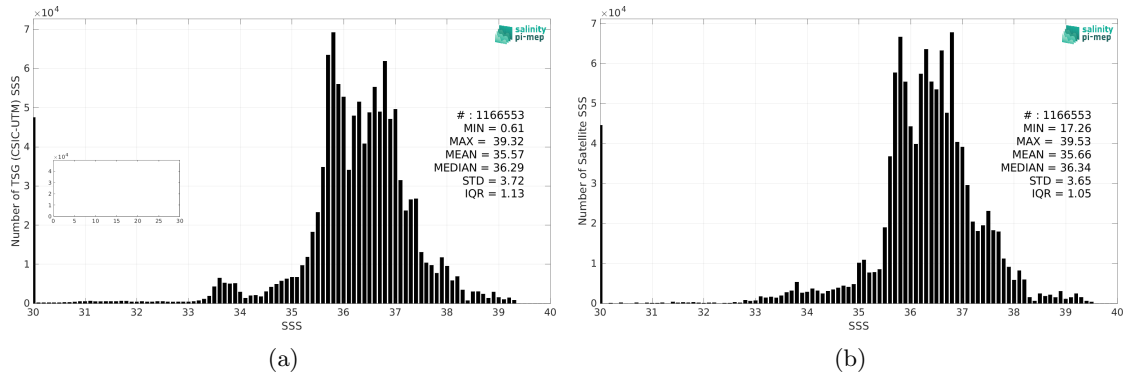
Figure 2: Histograms of SSS from TSG (CSIC-UTM) (a) and SMAP SSS L4 OI v2 - 7 Days (ESR) (b) considering all match-up pairs per bins of 0.1 over the Mid-Low Latitudes 45N-45S Pi-MEP region and for the full satellite product period.
