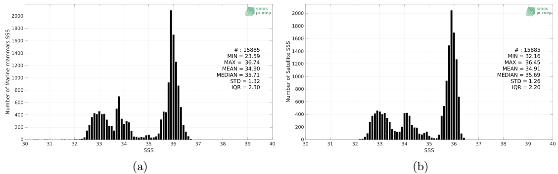
Figure 2: Histograms of SSS from Marine mammals (a) and SMAP SSS L4 OI v2 - 7 Days (ESR) (b) considering all match-up pairs per bins of 0.1 over the Mid-Low Latitudes 45N-45S Pi-MEP region and for the full satellite product period.
