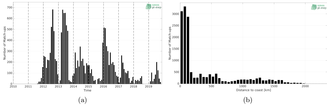
Figure 1: Number of match-ups between Marine mammals and SMAP SSS L4 OI v2 - 7 Days (ESR) SSS as a function of time (a) and as function of the distance to coast (b) over the Mid-Low Latitudes 45N-45S Pi-MEP region and for the full satellite product period.
