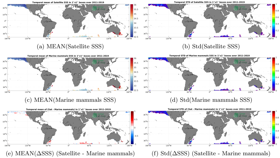
Figure 6: Temporal mean (left) and Std (right) of SSS from SMAP SSS L4 OI v2 - 7 Days (ESR) (top), Marine mammals (middle), and of \Delta SSS (Satellite - Marine mammals). Only match-up pairs are used to generate these maps.
