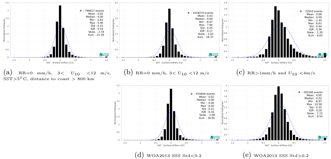
Figure 12: Normalized histogram of \Delta SSS (SMAP SSS L4 OI v2 - 7 Days (ESR) - Surface drifters) for 5 different subdatasets corresponding to: RR=0 mm/h, 3 < U_{10} < 12 m/s, SST >5^\circ\text{C} , distance to coast > 800 km (a), RR=0 mm/h, 3 < U_{10} < 12 m/s (b), RR >1 mm/h and U_{10} < 4 m/s (c), WOA2013 SSS Std <0.2 (d), WOA2013 SSS Std >0.2 (e).
