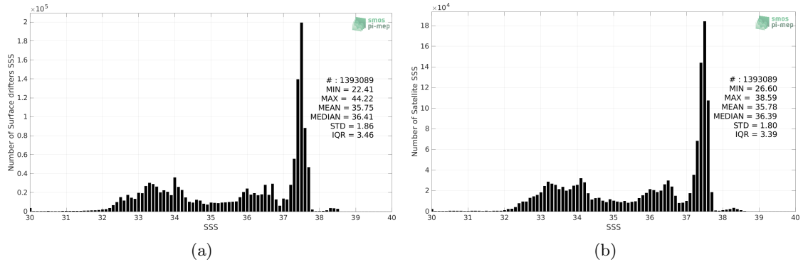
Figure 2: Histograms of SSS from Surface drifters (a) and SMAP SSS L4 OI v2 - 7 Days (ESR) (b) considering all match-up pairs per bins of 0.1 over the Mid-Low Latitudes 45N-45S Pi-MEP region and for the full satellite product period.
