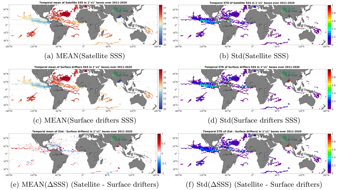
Figure 5: Temporal mean (left) and Std (right) of SSS from SMAP SSS L4 OI v2 - 7 Days (ESR) (top), Surface drifters (middle), and of \Delta SSS (Satellite - Surface drifters). Only match-up pairs are used to generate these maps.
