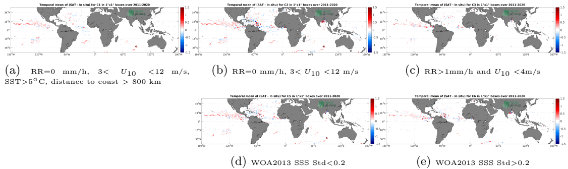
Figure 11: Temporal mean gridded over spatial boxes of size 1^\circ \times 1^\circ of \Delta SSS (SMAP SSS L4 OI v2 - 7 Days (ESR) - Surface drifters) for 5 different subdatasets corresponding to:RR=0 mm/h, 3 < U_{10} < 12 m/s, SST>5°C, distance to coast > 800 km (a), RR=0 mm/h, 3 < U_{10} < 12 m/s (b), RR>1mm/h and U_{10} < 4 m/s (c), WOA2013 SSS Std<0.2 (d), WOA2013 SSS Std>0.2 (e).
