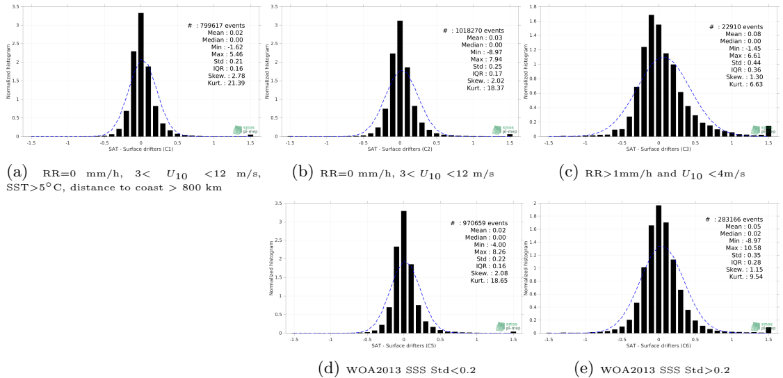
Figure 12: Normalized histogram of \Delta SSS (SMAP SSS L4 OI v2 - 7 Days (ESR) - Surface drifters) for 5 different subdatasets corresponding to: RR=0 mm/h, 3 < U_{10} < 12 m/s, SST>5°C, distance to coast > 800 km (a), RR=0 mm/h, 3 < U_{10} < 12 m/s (b), RR>1mm/h and U_{10} < 4 m/s (c), WOA2013 SSS Std<0.2 (d), WOA2013 SSS Std>0.2 (e).
