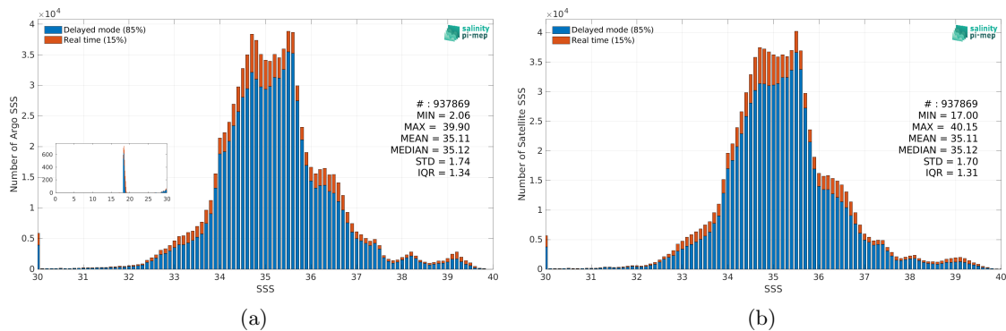
Figure 2: Histograms of SSS from Argo (a) and SMAP SSS L4 OI v2 - 7 Days (ESR) (b) considering all match-up pairs per bins of 0.1 over the Mid-Low Latitudes 45N-45S Pi-MEP region and for the full satellite product period.
