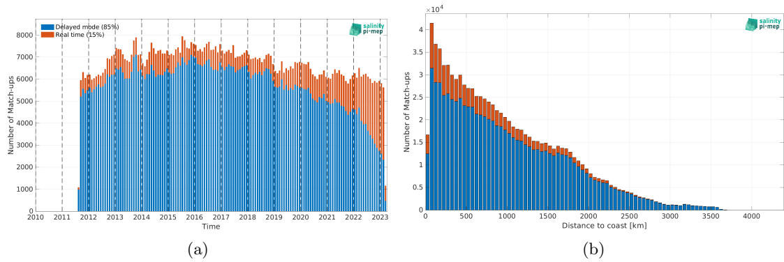
Figure 1: Number of match-ups between Argo and SMAP SSS L4 OI v2 - 7 Days (ESR) SSS as a function of time (a) and as function of the distance to coast (b) over the Mid-Low Latitudes 45N-45S Pi-MEP region and for the full satellite product period.
