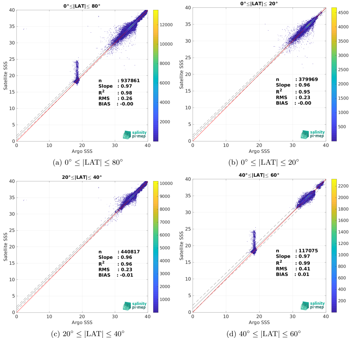
Figure 9: Contour maps of the concentration of SMAP SSS L4 OI v2 - 7 Days (ESR) SSS (y-axis) versus Argo SSS (x-axis) at match-up pairs for different latitude bands. For each plot, the red line shows x=y . The black thin and dashed lines indicate a linear fit through the data cloud and the \pm 95\% confidence levels, respectively. The number match-up pairs n , the slope and R^2 coefficient of the linear fit, the root mean square (RMS) and the mean bias between satellite and in situ data are indicated for each latitude band in each plots.
