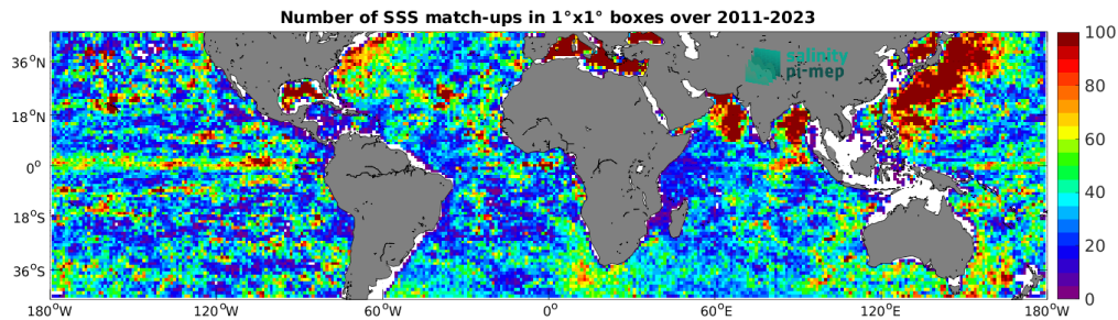
Figure 4: Number of SSS match-ups between Argo SSS and the SMAP SSS L4 OI v2 - 7 Days (ESR) SSS product for the Mid-Low Latitudes 45N-45S Pi-MEP region over 1^\circ \times 1^\circ boxes and for the full satellite product period.
