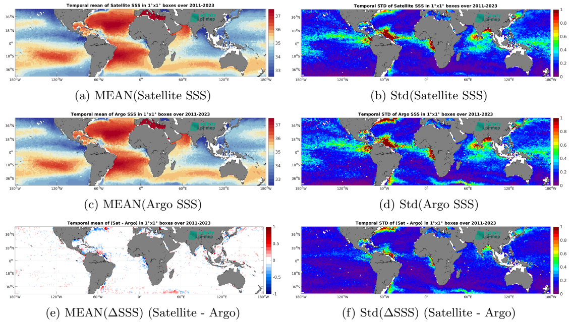
Figure 6: Temporal mean (left) and Std (right) of SSS from SMAP SSS L4 OI v2 - 7 Days (ESR) (top), Argo (middle), and of \Delta SSS (Satellite - Argo). Only match-up pairs are used to generate these maps.
