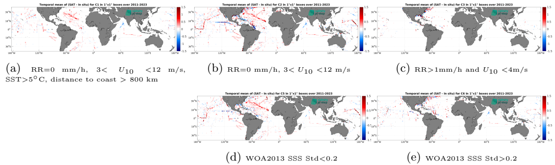
Figure 12: Temporal mean gridded over spatial boxes of size 1^\circ \times 1^\circ of \Delta SSS (SMAP SSS L4 OI v2 - Monthly (IPRC) - TSG (SAMOS)) for 5 different subdatasets corresponding to: RR=0 mm/h, 3 < U_{10} < 12 m/s, SST > 5°C, distance to coast > 800 km (a), RR=0 mm/h, 3 < U_{10} < 12 m/s (b), RR > 1mm/h and U_{10} < 4 m/s (c), WOA2013 SSS Std < 0.2 (d), WOA2013 SSS Std > 0.2 (e).
