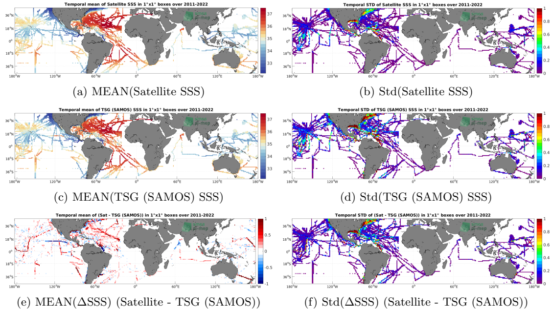
Figure 6: Temporal mean (left) and Std (right) of SSS from SMAP SSS L4 OI v2 - Monthly (IPRC) (top), TSG (SAMOS) (middle), and of \Delta SSS (Satellite - TSG (SAMOS)). Only match-up pairs are used to generate these maps.
