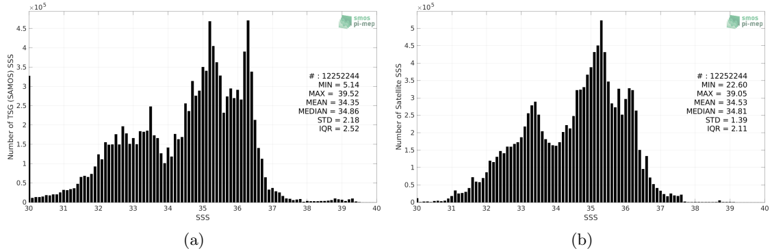
Figure 2: Histograms of SSS from TSG (SAMOS) (a) and SMAP SSS L4 OI v2 - Monthly (IPRC) (b) considering all match-up pairs per bins of 0.1 over the Mid-Low Latitudes 45N-45S Pi-MEP region and for the full satellite product period.
