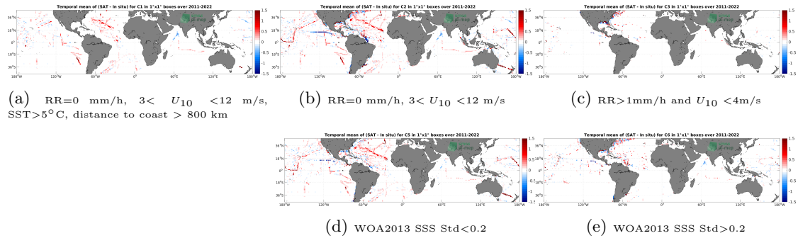
Figure 12: Temporal mean gridded over spatial boxes of size 1^\circ \times 1^\circ of \Delta SSS (SMAP SSS L4 OI v2 - Monthly (IPRC) - TSG (SAMOS)) for 5 different subdatasets corresponding to:RR=0 mm/h, 3 < U_{10} < 12 m/s, SST >5^\circ\text{C} , distance to coast > 800 km (a), RR=0 mm/h, 3 < U_{10} < 12 m/s (b), RR >1 mm/h and U_{10} < 4 m/s (c), WOA2013 SSS Std <0.2 (d), WOA2013 SSS Std >0.2 (e).
