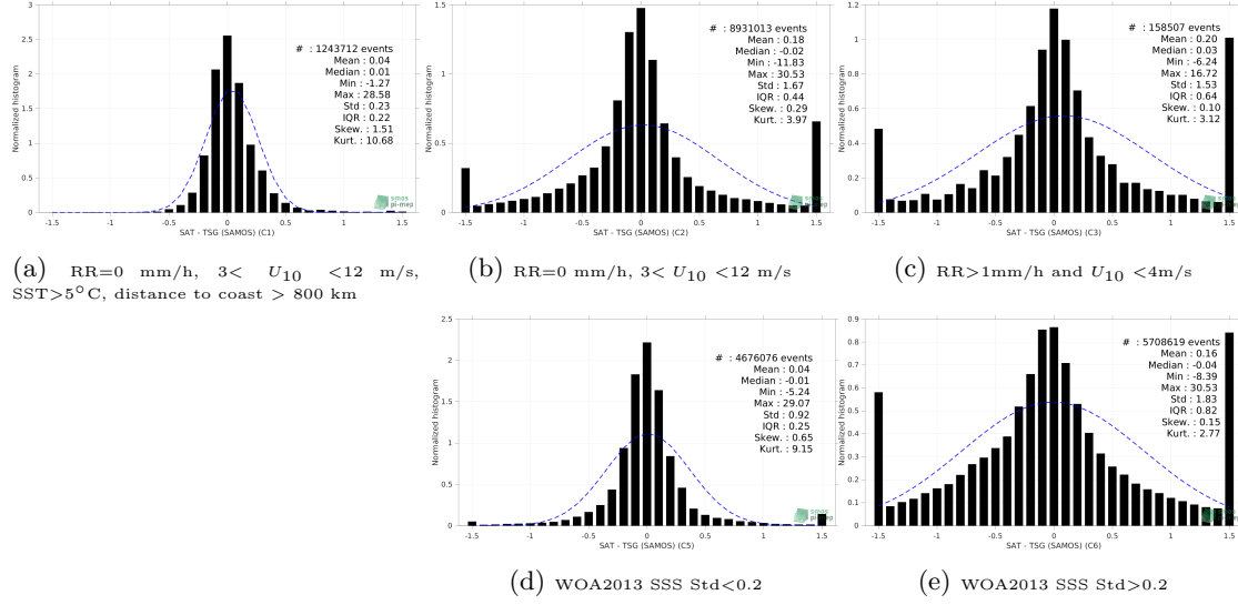
Figure 13: Normalized histogram of \Delta SSS (SMAP SSS L4 OI v2 - Monthly (IPRC) - TSG (SAMOS)) for 5 different subdatasets corresponding to: RR=0 mm/h, 3 < U_{10} < 12 m/s, SST>5°C, distance to coast > 800 km (a), RR=0 mm/h, 3 < U_{10} < 12 m/s (b), RR>1mm/h and U_{10} < 4 m/s (c), WOA2013 SSS Std<0.2 (d), WOA2013 SSS Std>0.2 (e).
