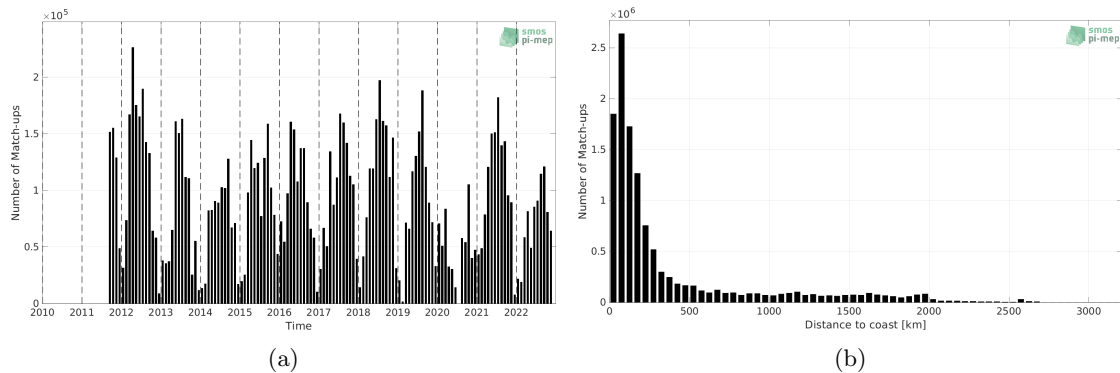
Figure 1: Number of match-ups between TSG (SAMOS) and SMAP SSS L4 OI v2 - Monthly (IPRC) SSS as a function of time (a) and as function of the distance to coast (b) over the Mid-Low Latitudes 45N-45S Pi-MEP region and for the full satellite product period.
